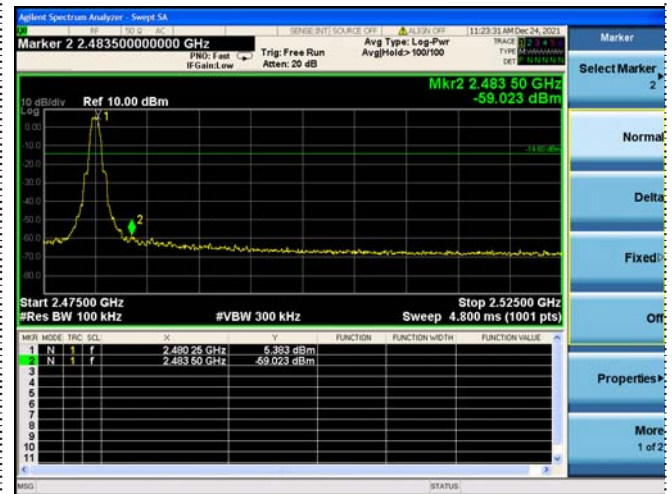
Right bandedge
