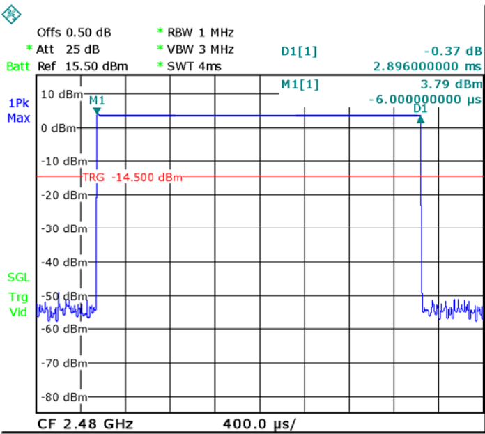
DH5.High channel
