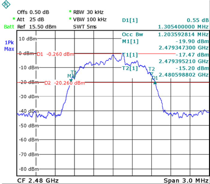
High Channel
