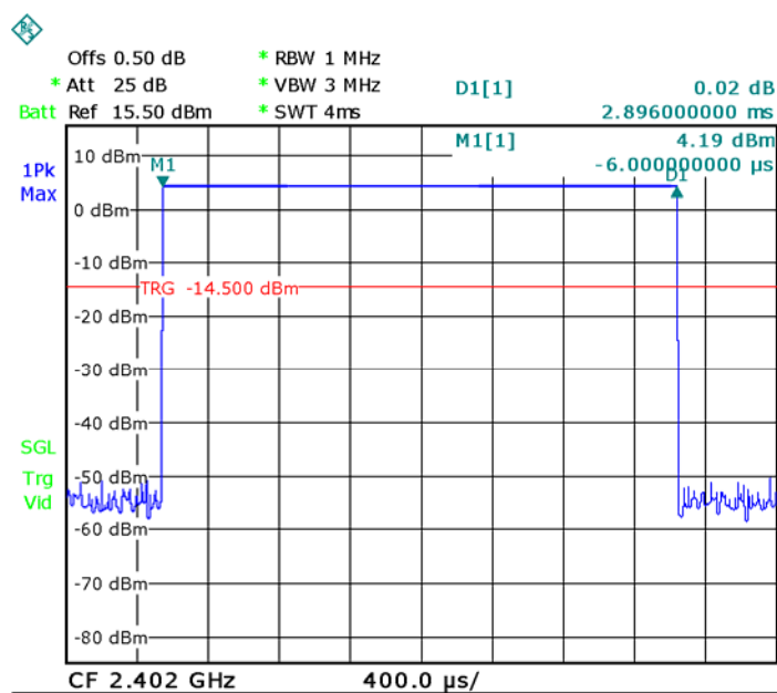
DH5.Low channel
