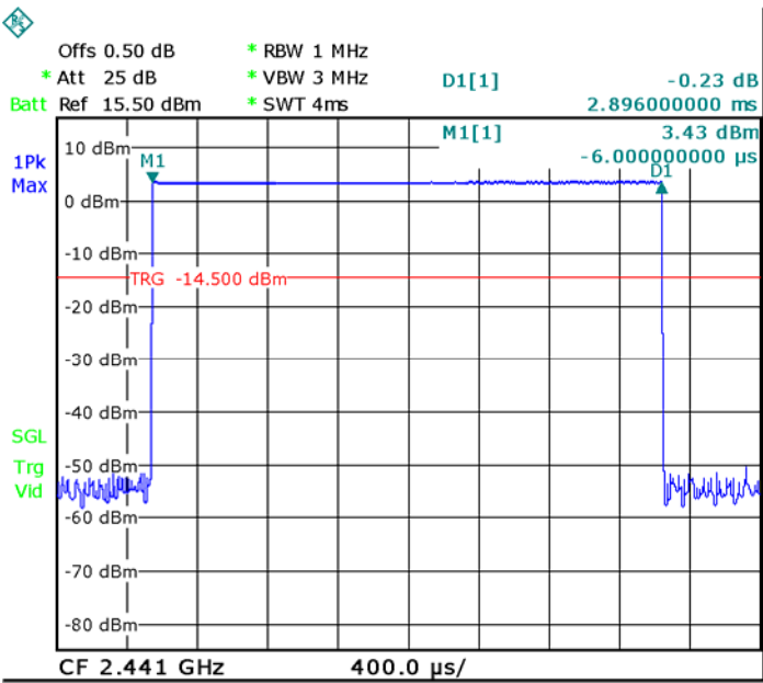
DH5.Middle channel
