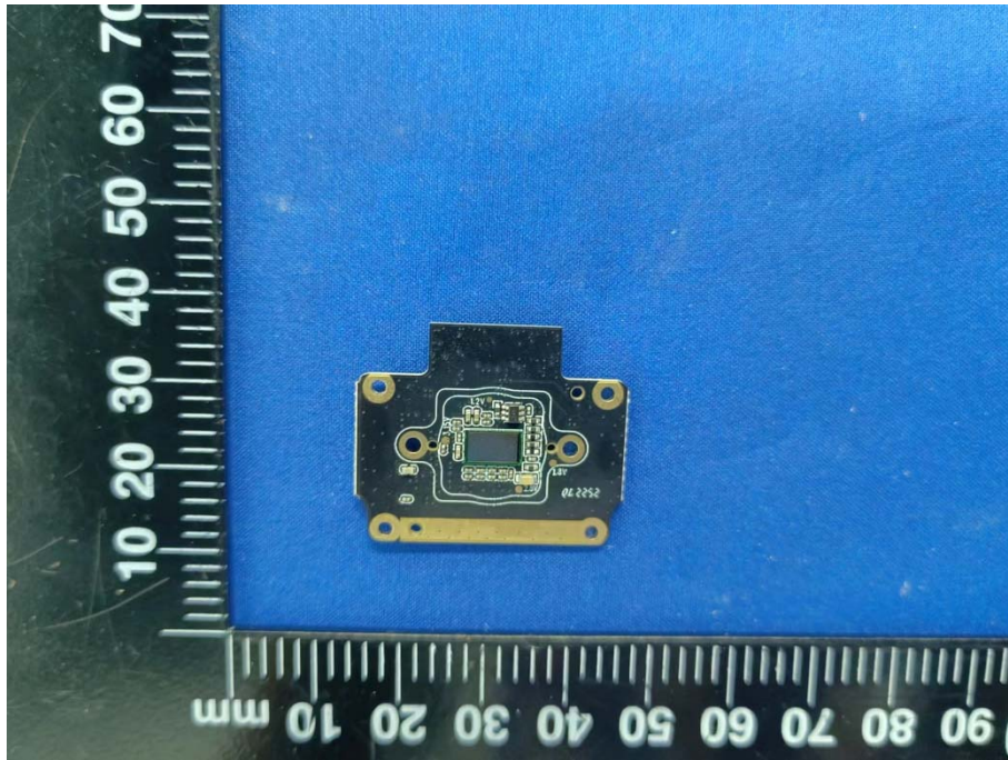
SUB BOARD REAR VIEW 2
