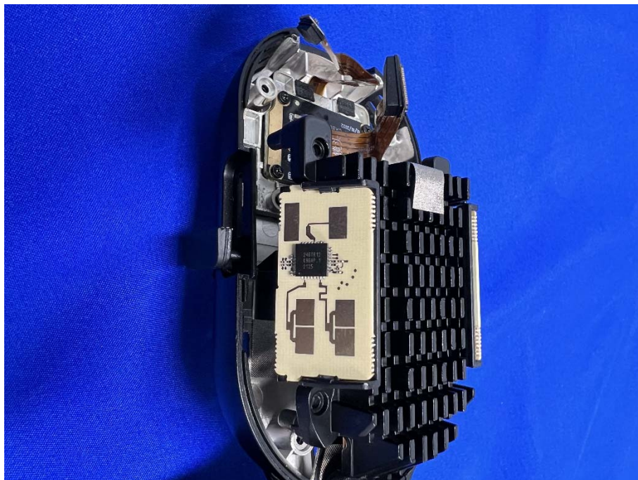
RADAR ANTENNA 1
