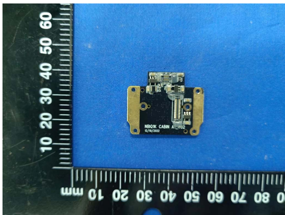
SUB BOARD TOP VIEW 2
