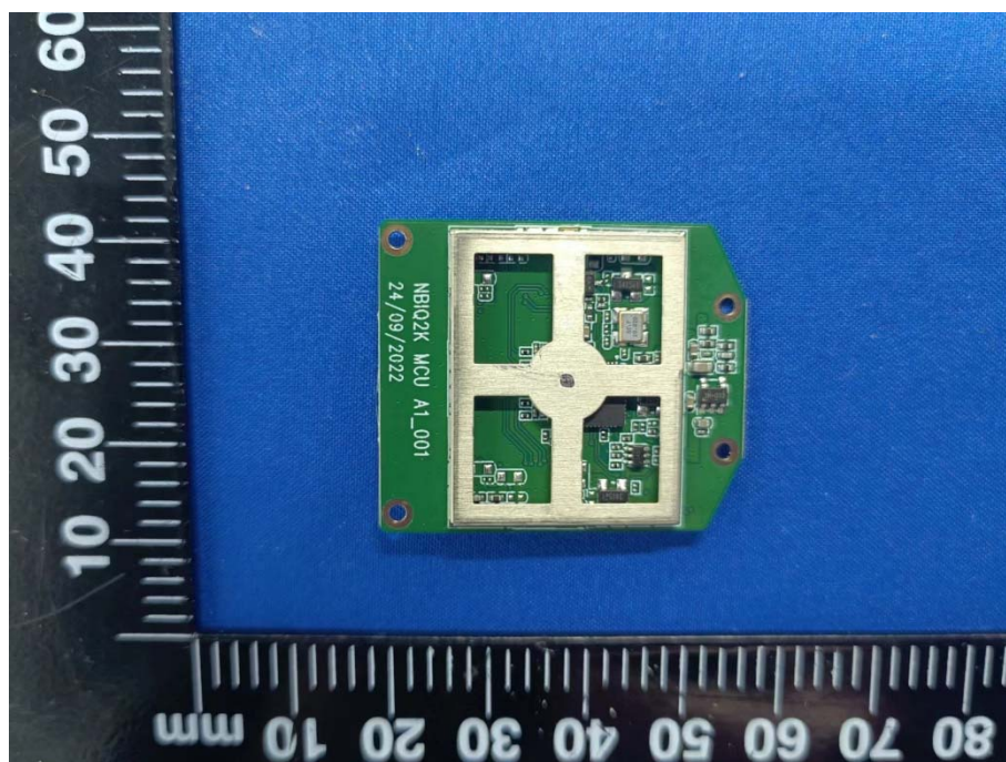
MAIN BOARD TOP VIEW 3 (WITH SHIELDING)
