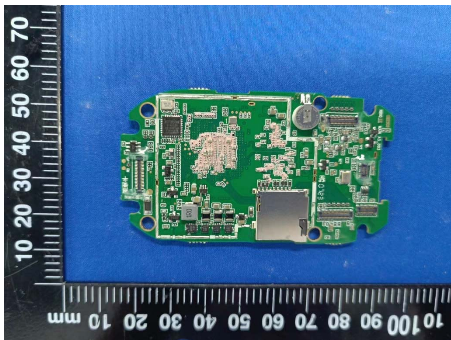
MAIN BOARD TOP VIEW 4 (WITHOUT SHIELDING)
