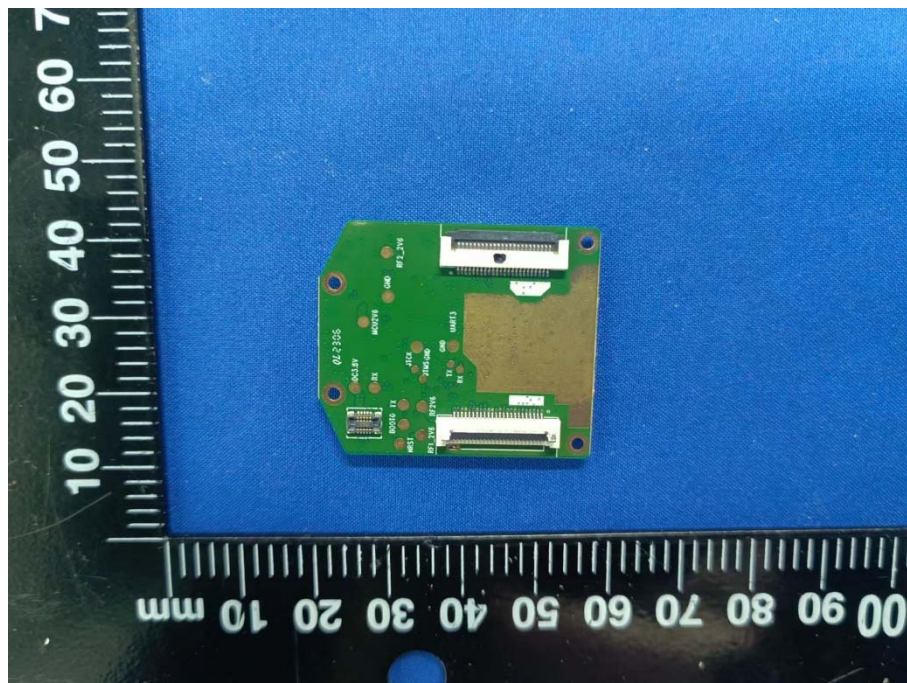
MAIN BOARD REAR VIEW 3 (WITHOUT SHIELDING)
