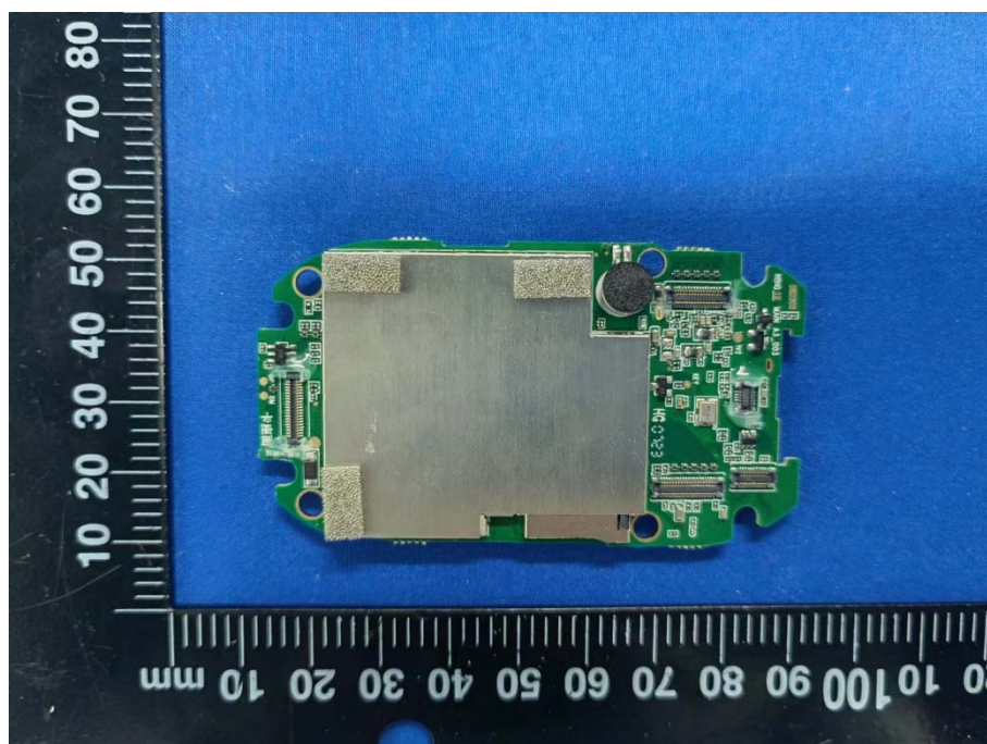
MAIN BOARD TOP VIEW 4 (WITH SHIELDING)
