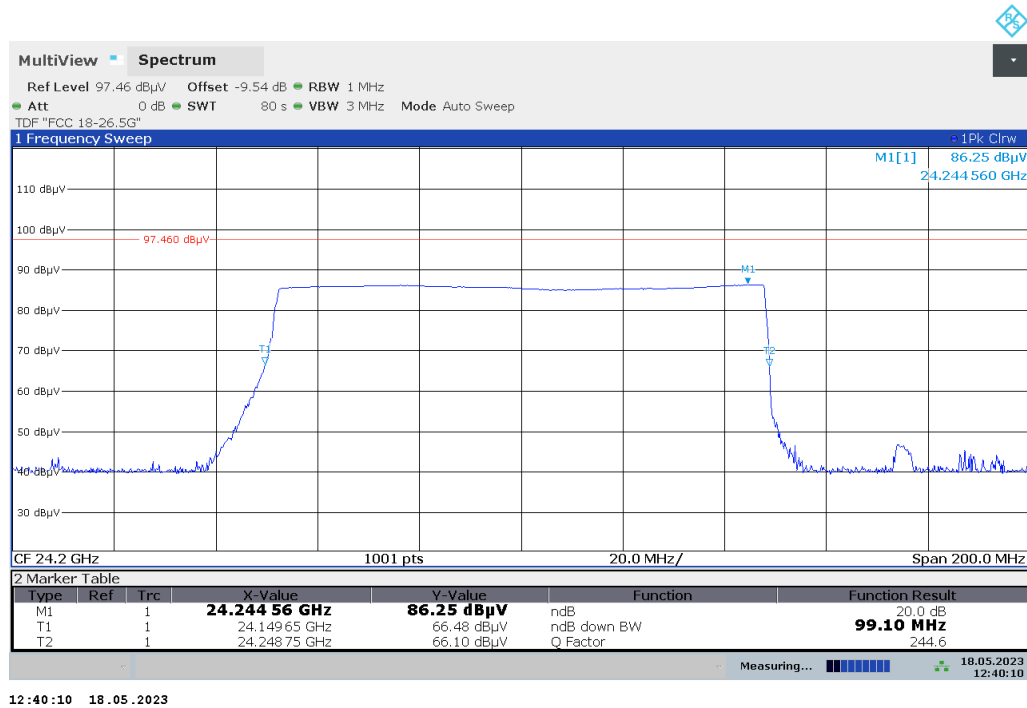
Plots No. 11: 20dB Bandwidth, Horizontal / Vertical Polarization
