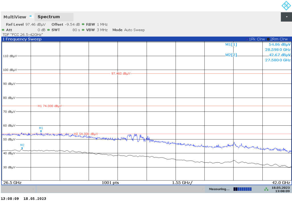
Plots No. 6: 26.5 GHz to 42 GHz, Horizontal / Vertical Polarization
