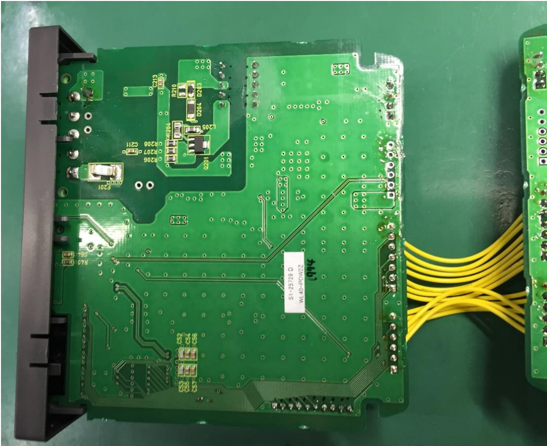
DC24V model (WL40EW2F-R)
