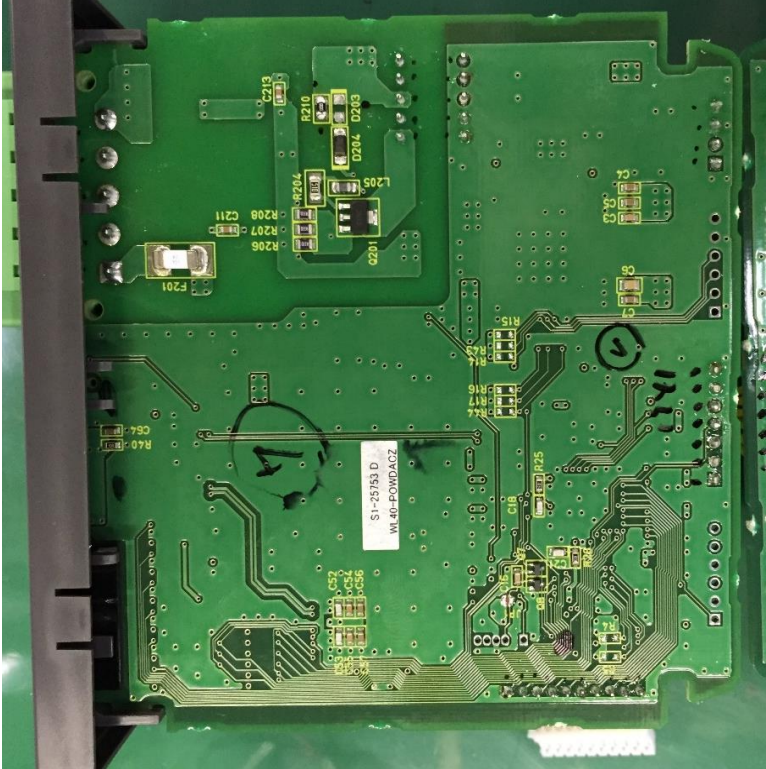
DC12V model (WL40W1F-DAC4A-S)
