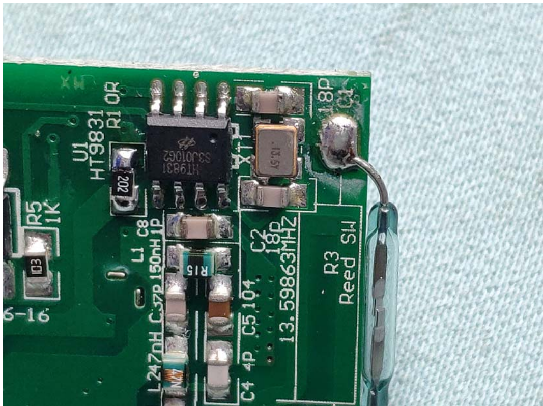
FIGURE 11 IDC CONSOLE (M/N: IDC CONSOLE) CRYSTAL#2 ON MAIN BOARD
