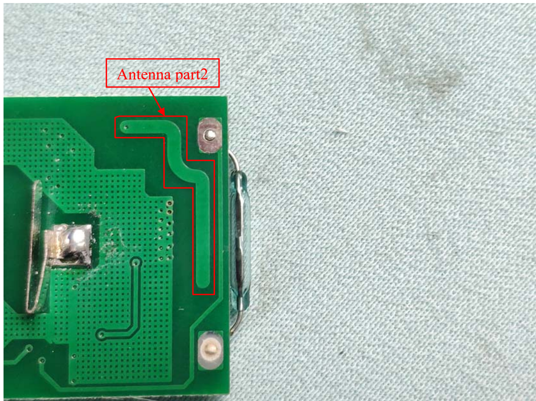
FIGURE 13 IDC CONSOLE (M/N: IDC CONSOLE) ANTENNA PART2
