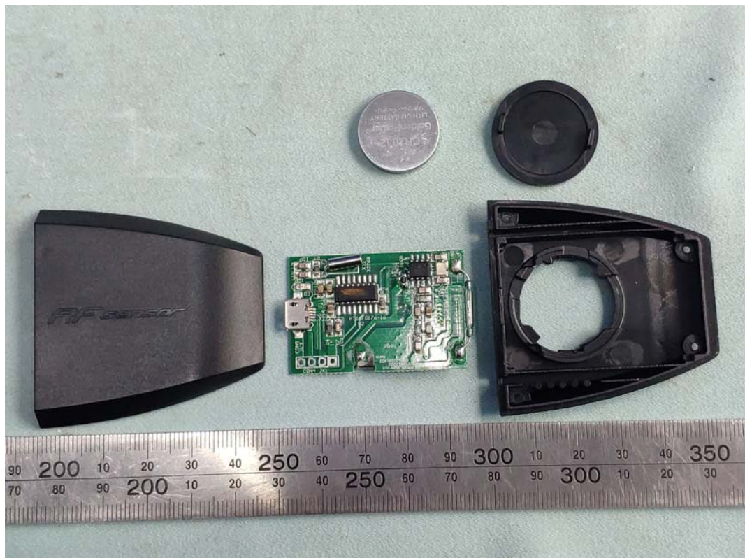
FIGURE 7 IDC CONSOLE (M/N: IDC CONSOLE) COVER REMOVED
