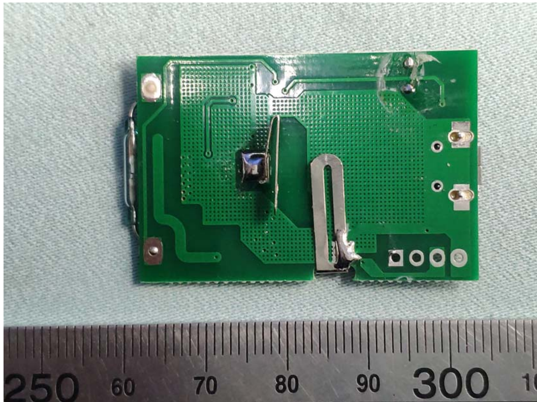
FIGURE 9 IDC CONSOLE (M/N: IDC CONSOLE) MAIN BOARD(BACK VIEW)
