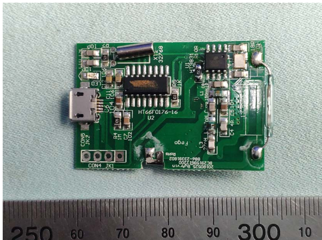
FIGURE 8 IDC CONSOLE (M/N: IDC CONSOLE) MAIN BOARD(FRONT VIEW)
