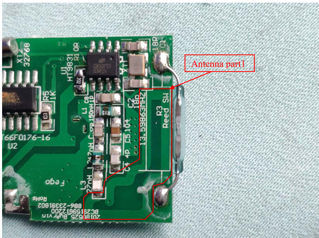
FIGURE 12 IDC CONSOLE (M/N: IDC CONSOLE) ANTENNA PART1
