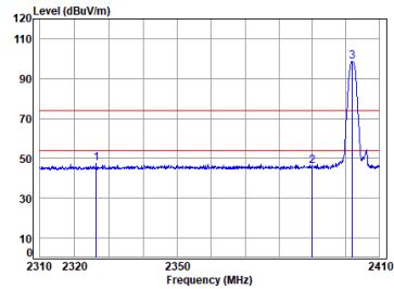
BT_DH5_TX_CH_00_Vertical
