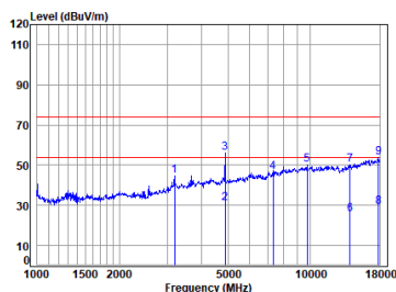
BT_DH5_TX_CH_39_Vertical
