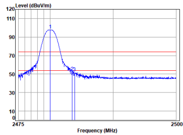
BT_DH5_TX_CH_78_Vertical
