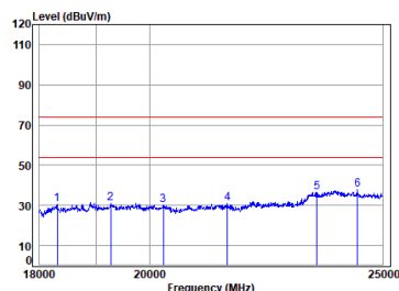
BT_DH5_TX_CH_00_Vertical
