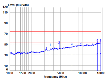
BT_DH5_TX_CH_00_Vertical
