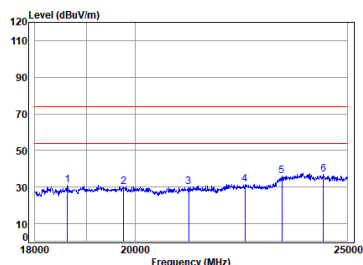
BT_DH5_TX_CH_00_Horizontal
