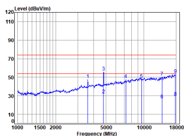
BT_DH5_TX_CH_00_Horizontal
