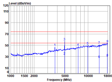
BT_DH5_TX_CH_78_Horizontal
