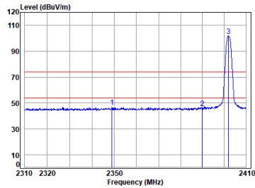
BT_DH5_TX_CH_00_Horizontal
