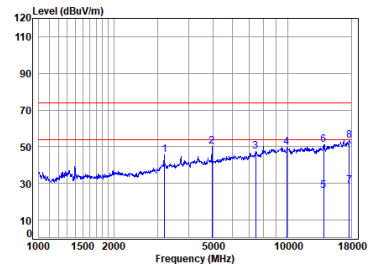
BT_DH5_TX_CH_78_Vertical
