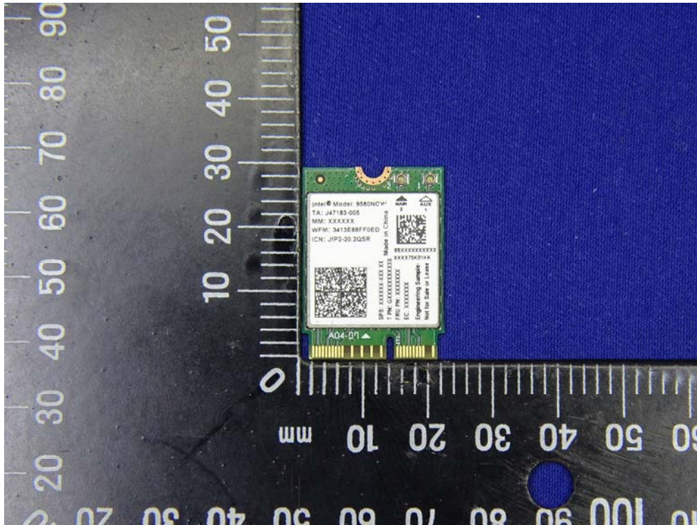
(1) EUT Photo
