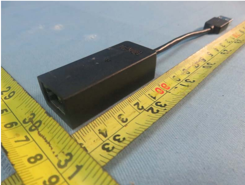
ThinkPad USB 3.0 Ethernet Adapter / RTL8153
