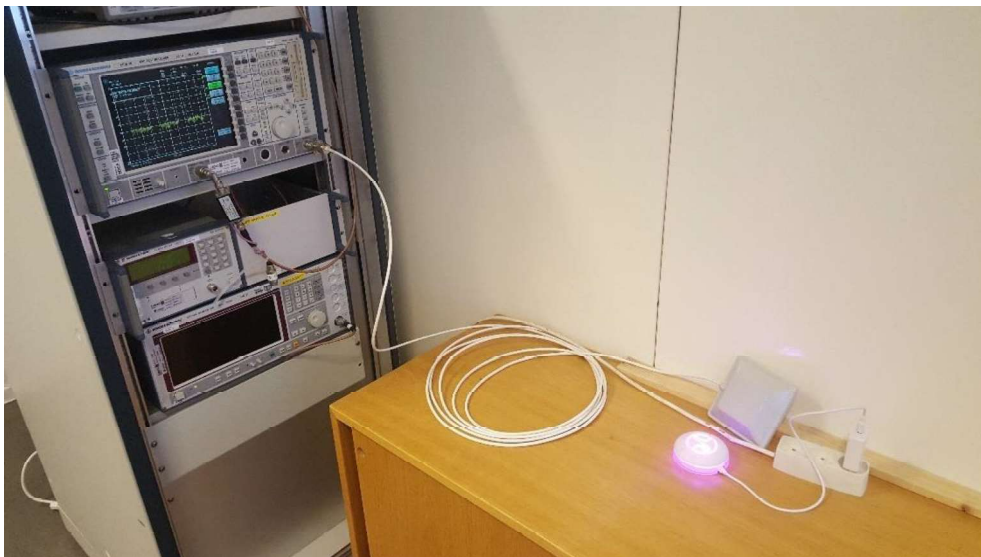
Photo 2. Duty cycle test set up.
