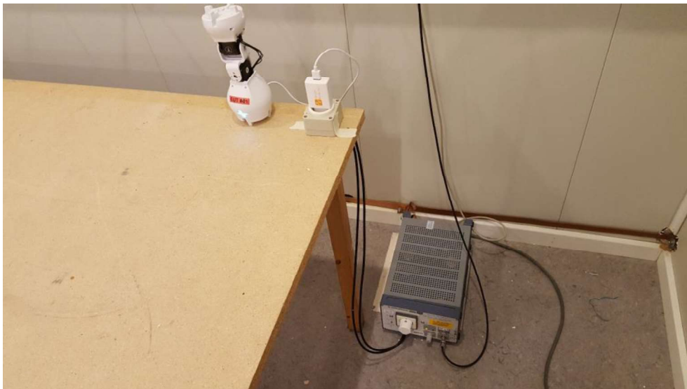
Photo 8. AC Conducted emission test set up.
