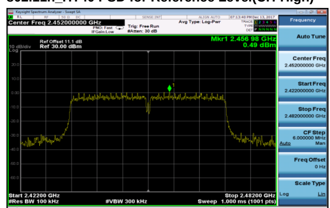
802.11n_HT40 PSD for Reference Level(CH-High)
