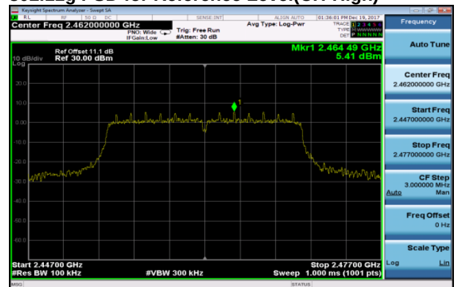
802.11g PSD for Reference Level (CH-High)
