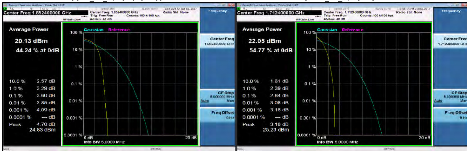
HSUPA_B2_LowCH9262-1852.4
