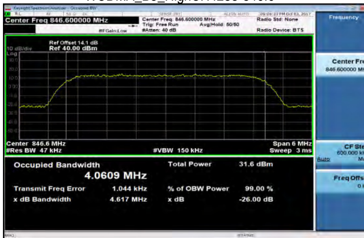
WCDMA_B5_HighCH4233-846.6
