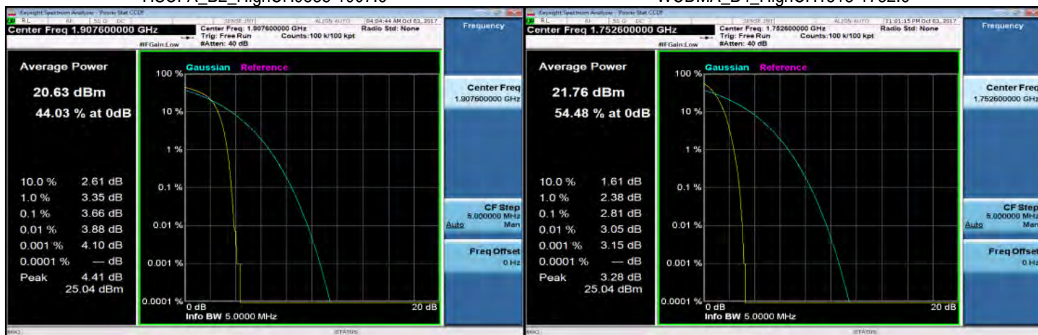
HSUPA_B2_HighCH9538-1907.6
