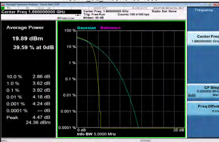
HSDPA_B2_MidCH9400-1880
