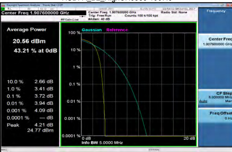
HSDPA_B2_HighCH9538-1907.6
