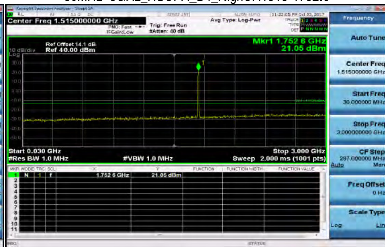
30MHz~3GHz_HSUPA_B4_HighCH1513-1752.6
