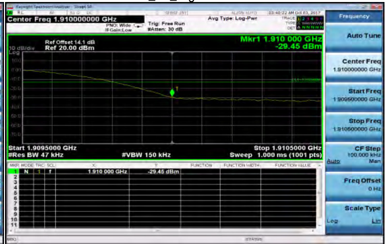
WCDMA_B2_HighCH9538-1907.6
