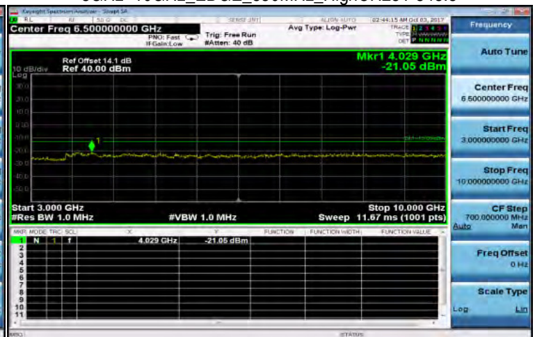
3GHz~10GHz_EDGE_850MHz_HighCH251-848.8
