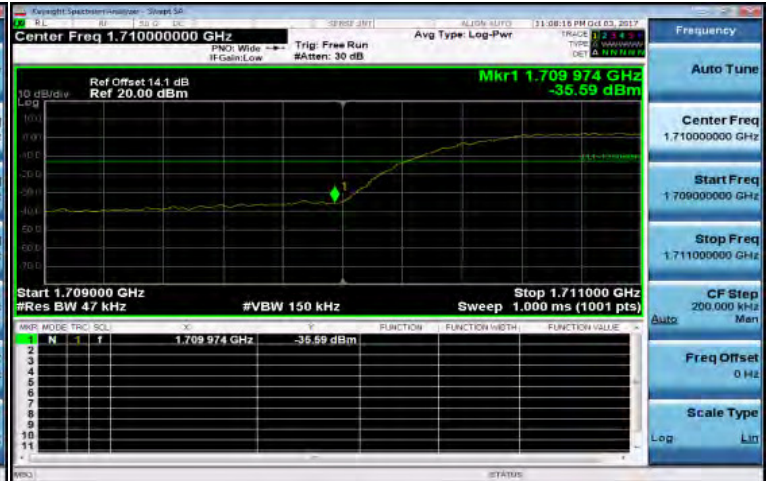
HSDPA_B4_LowCH1312-1712.4
