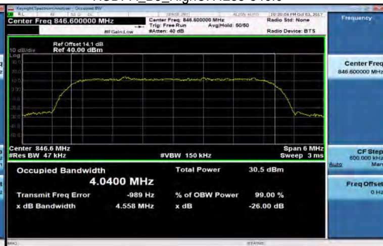
HSDPA_B5_HighCH4233-846.6
