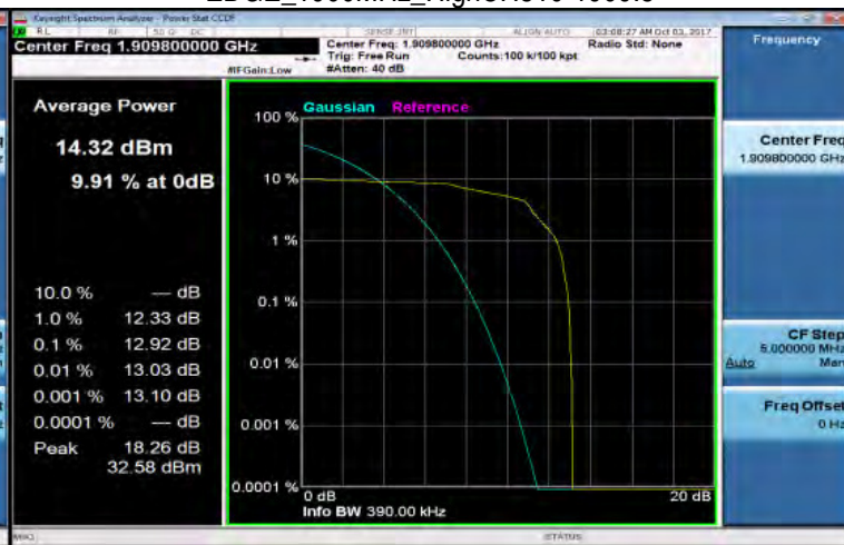
EDGE_1900MHz_HighCH810-1909.8
