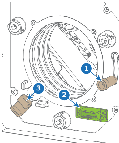
Image 5-10 Lens installation, preparation
