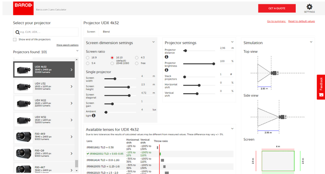
Image 5-9 Lens calculator
