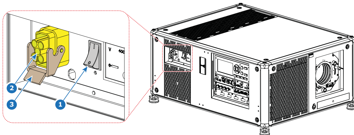
Image 4-1 Power input
