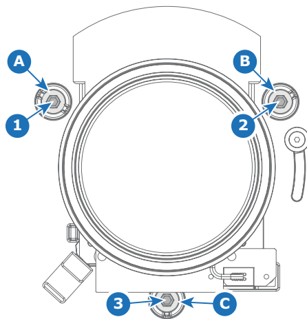
Image 5-18 Scheimpflug adjustments
