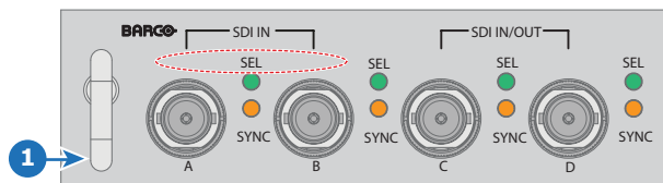
Image 6-7 3G V&H Input, without markings above the SDI inputs
