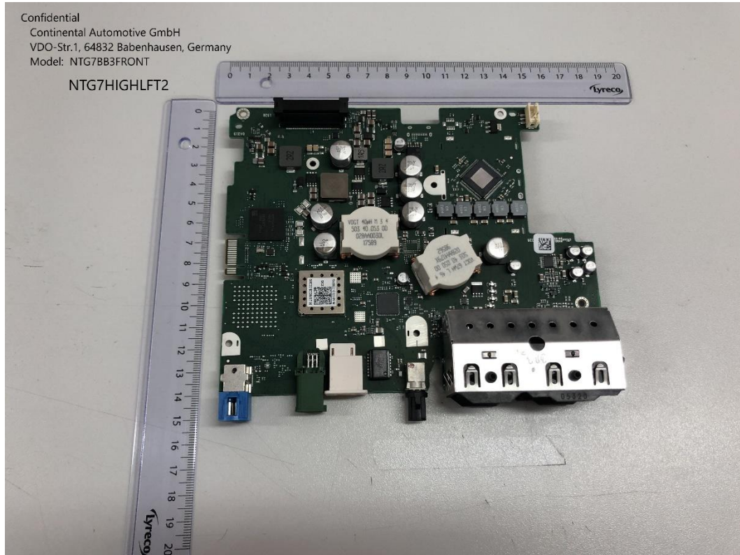
Base board 3 top view
