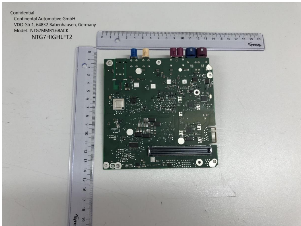
Multimedia board 1.6 bottom view
