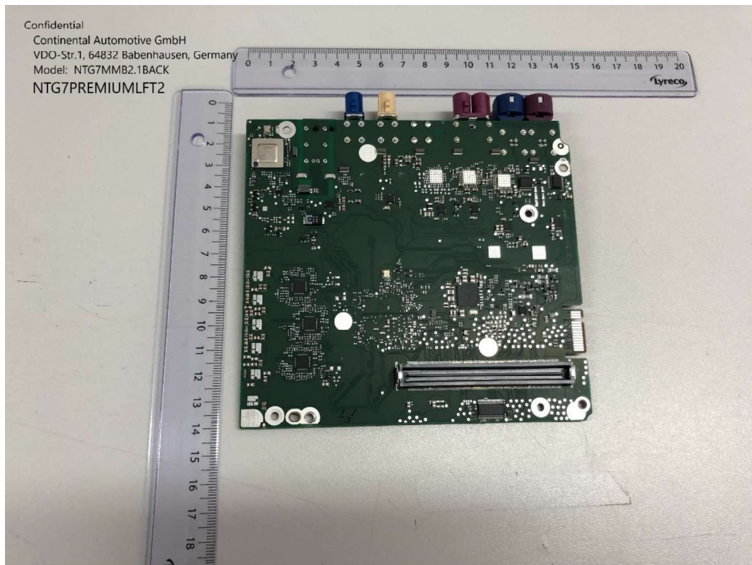
Multimedia board 2.1 bottom view
