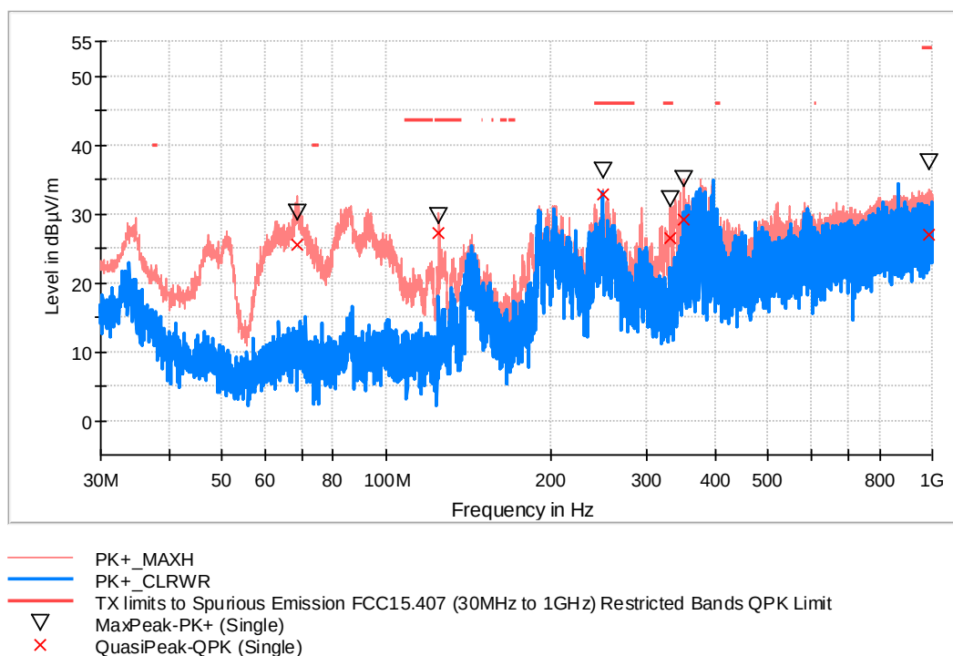
RF_FCC_15.407_E Field_30MHz_1GHz
