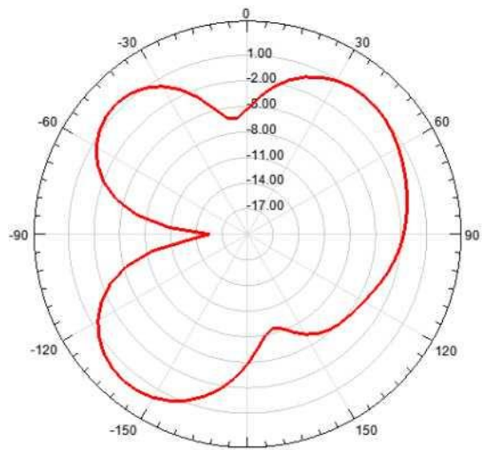
Radiation Pattern 2
