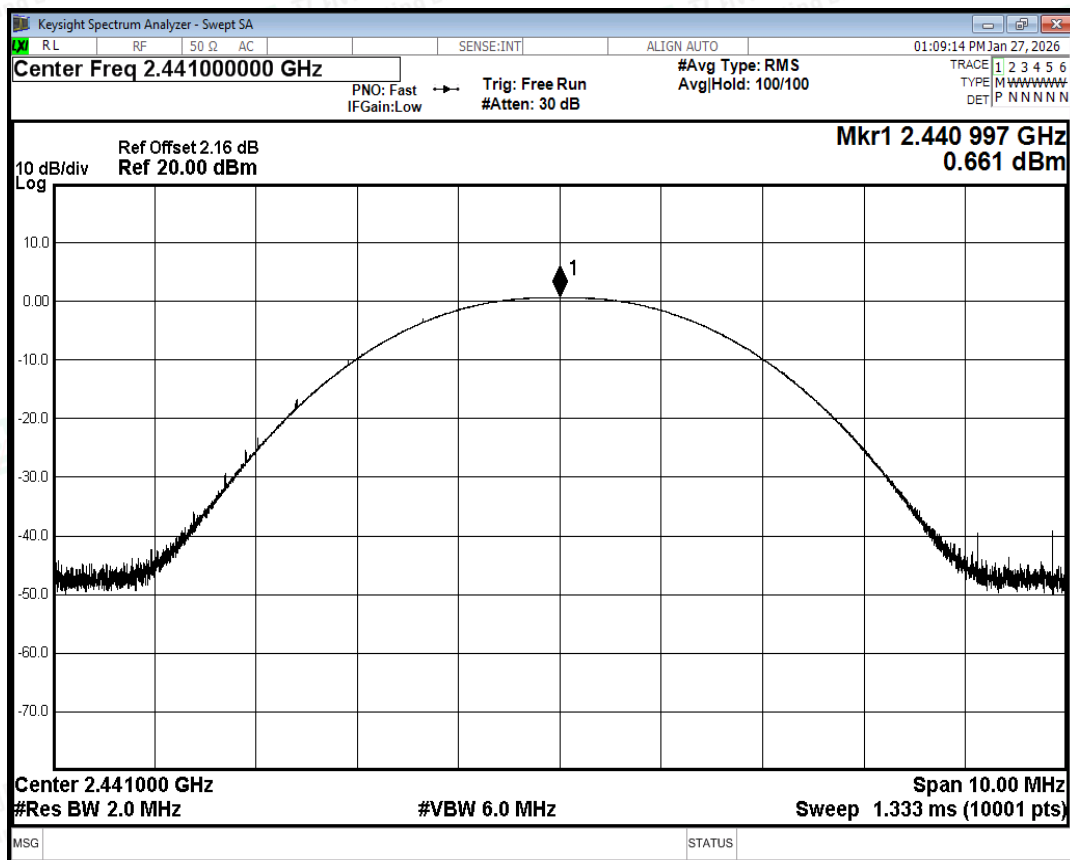
Peak Power NVNT 1-DH5 2441MHz Ant0
