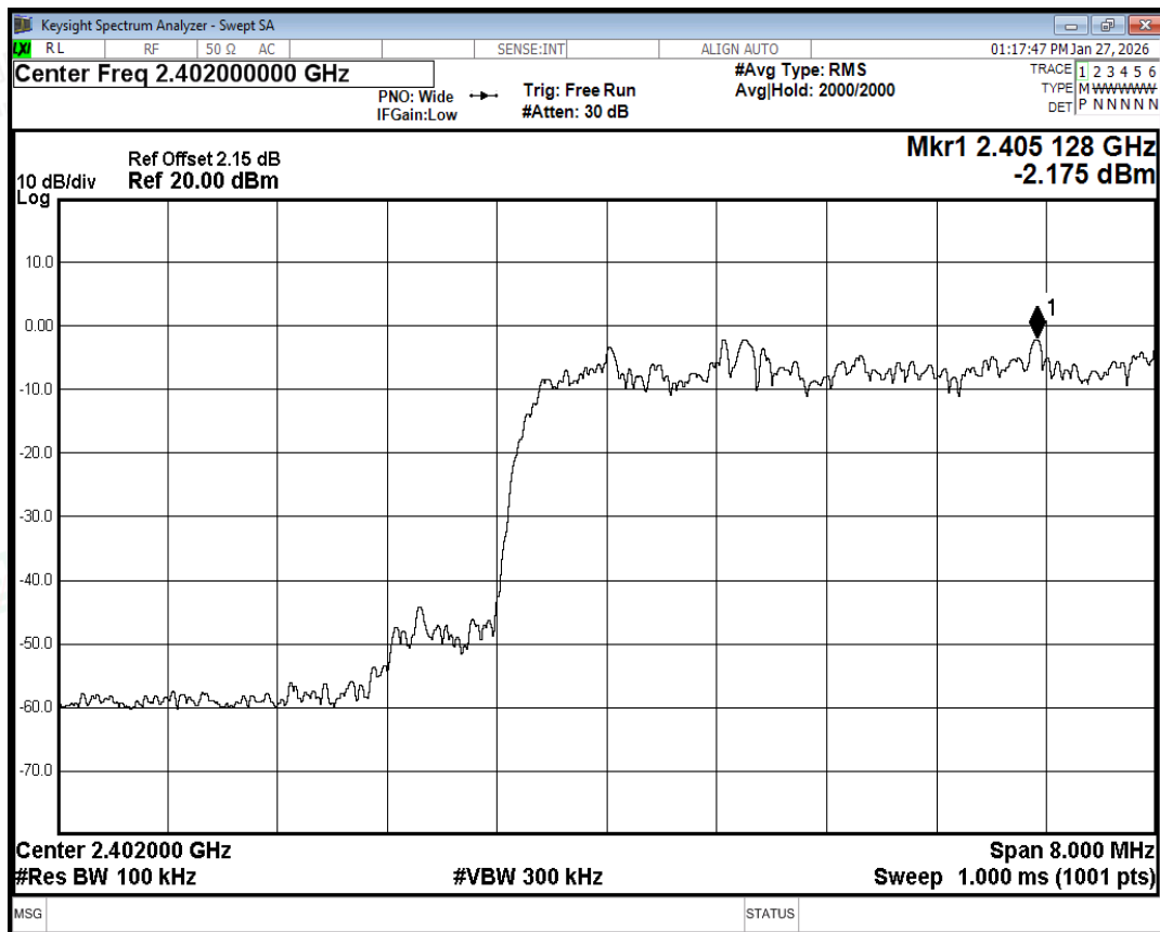
Band Edge(Hopping) NVNT 2-DH5 2402MHz Ant0 Hopping Ref
