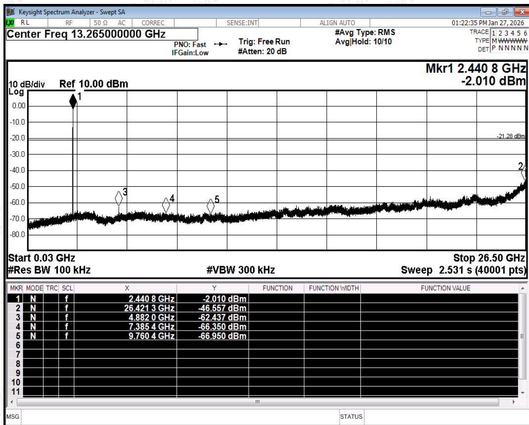
Tx. Spurious NVNT 2-DH5 2441MHz Ant0 Emission
