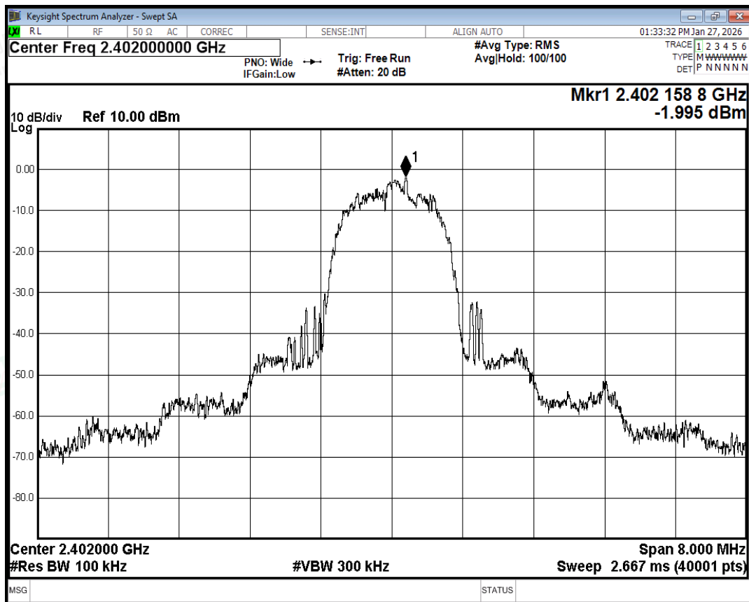
Tx. Spurious NVNT 3-DH5 2402MHz Ant0 Ref
