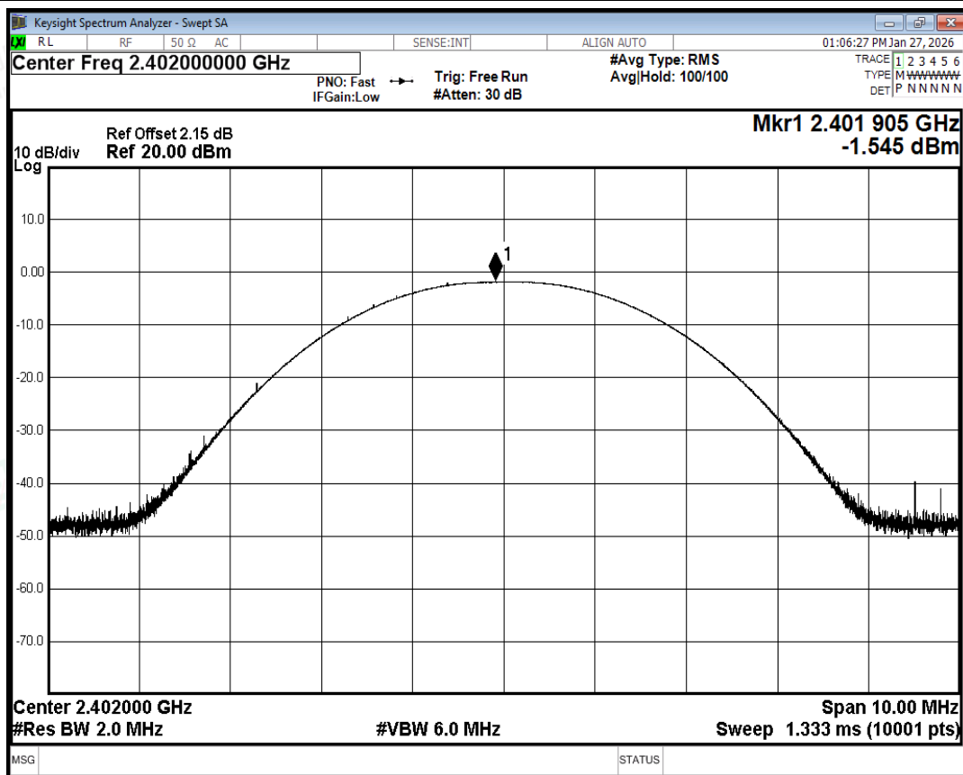
Peak Power NVNT 1-DH5 2402MHz Ant0
