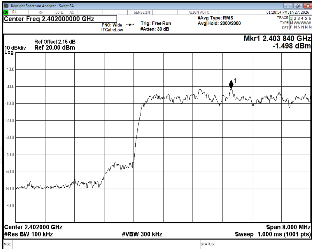
Band Edge(Hopping) NVNT 3-DH5 2402MHz Ant0 Hopping Ref
