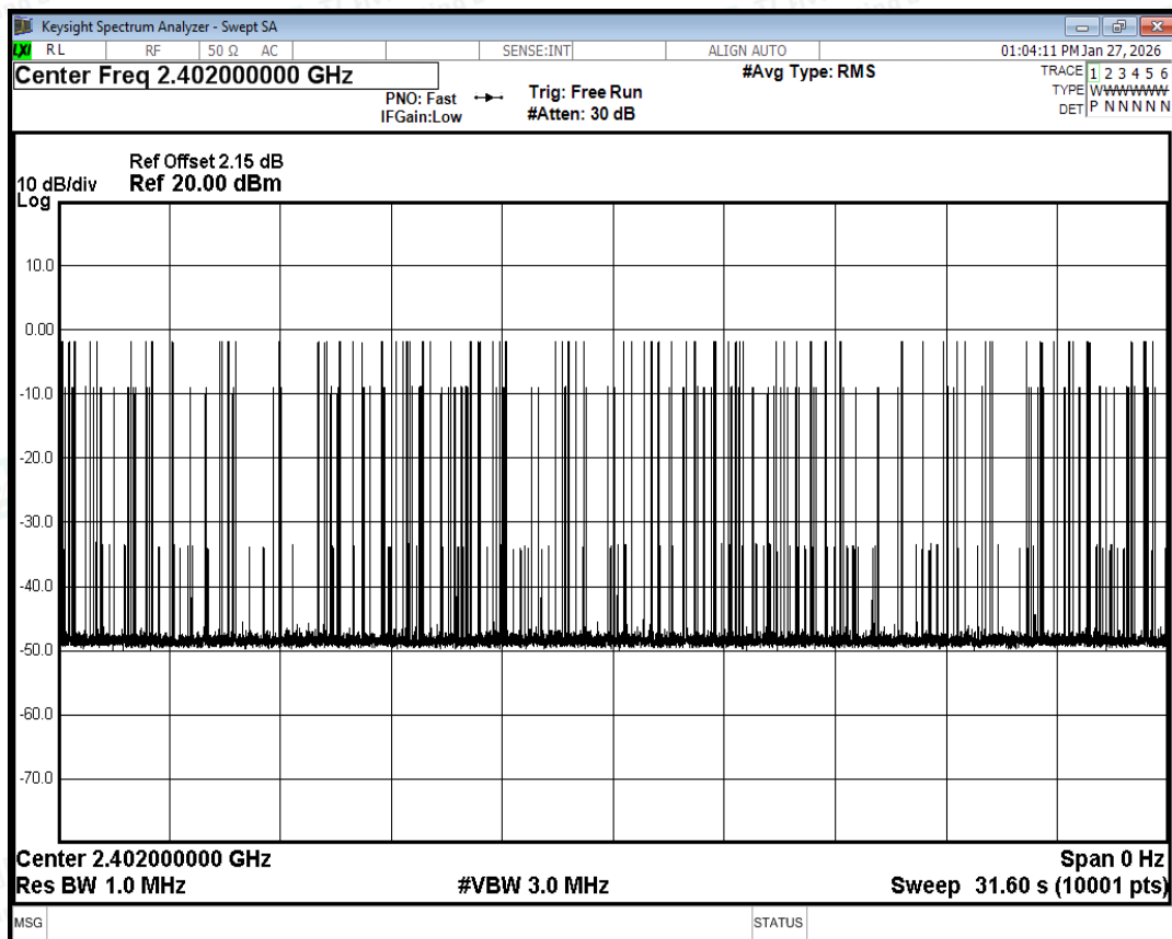
Dwell NVNT 1-DH5 2402MHz Ant0 Accumulated
