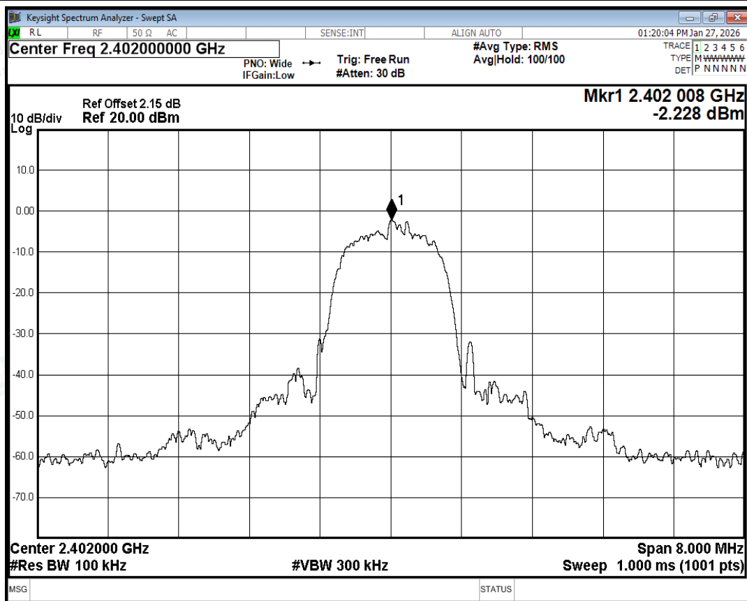
Band Edge NVNT 2-DH5 2402MHz Ant0 No-Hopping Ref
