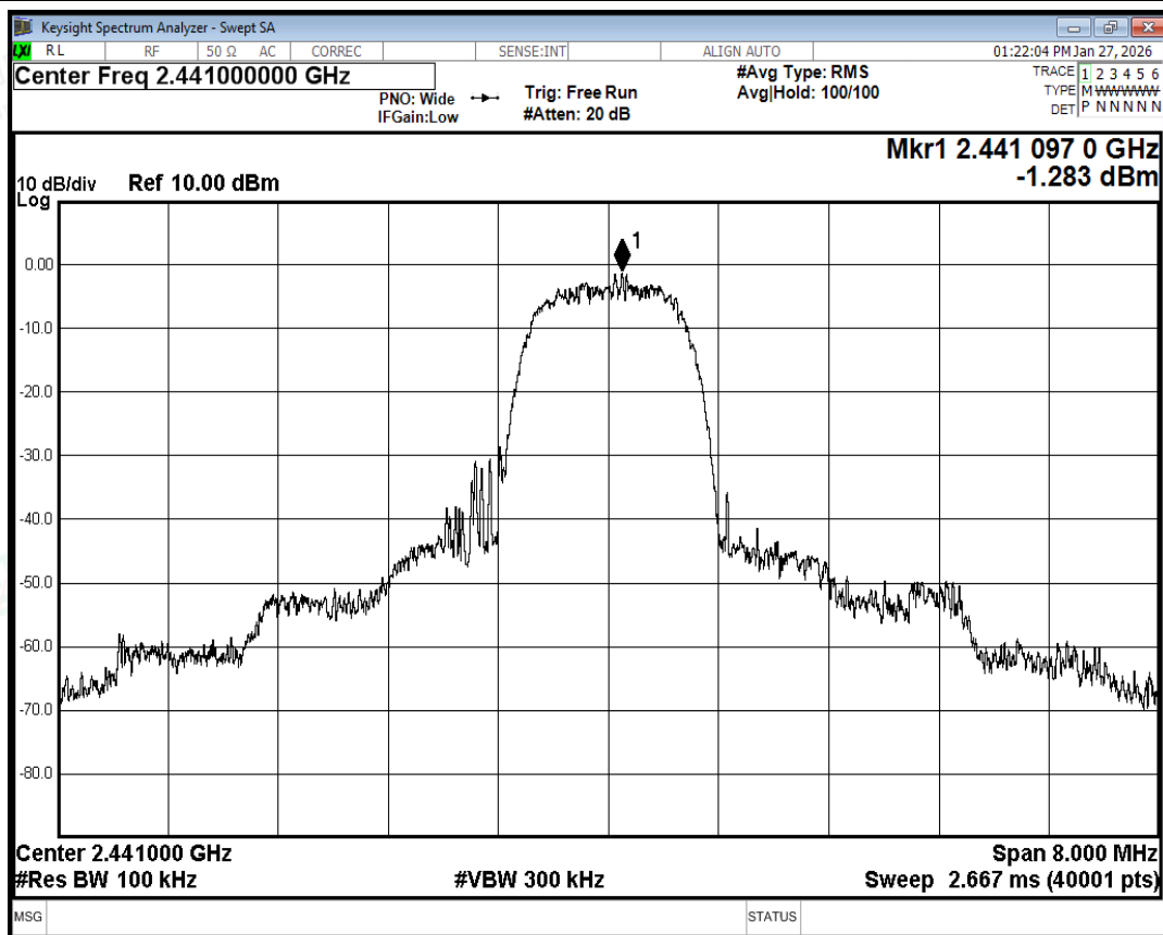
Tx. Spurious NVNT 2-DH5 2441MHz Ant0 Ref
