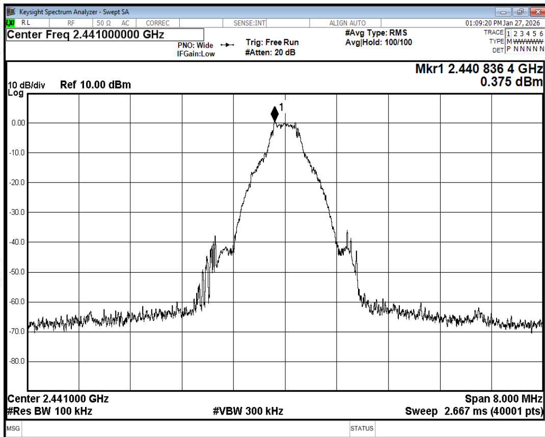
Tx. Spurious NVNT 1-DH5 2441MHz Ant0 Ref
