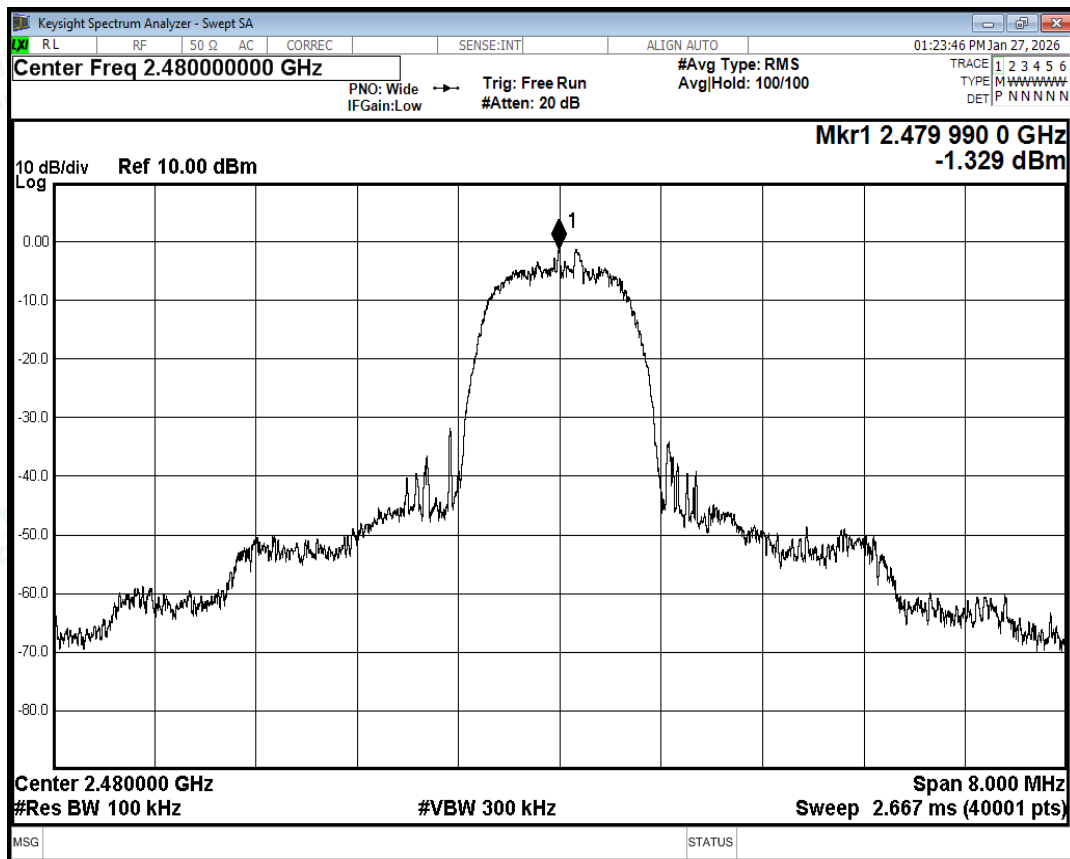
Tx. Spurious NVNT 2-DH5 2480MHz Ant0 Ref
