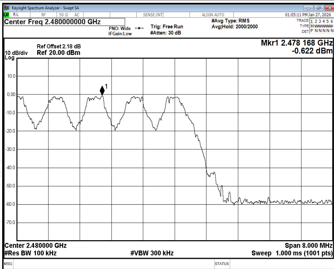
Band Edge(Hopping) NVNT 1-DH5 2480MHz Ant0 Hopping Ref
