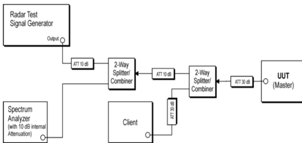
Figure 7-1. Test Setup
