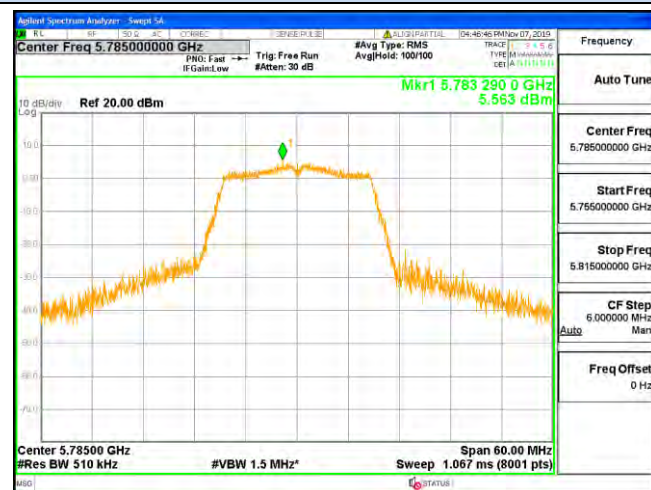
Channel 157 / 5785 MHz
