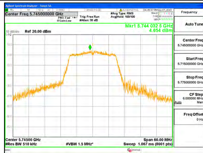
Channel 149 / 5745 MHz
