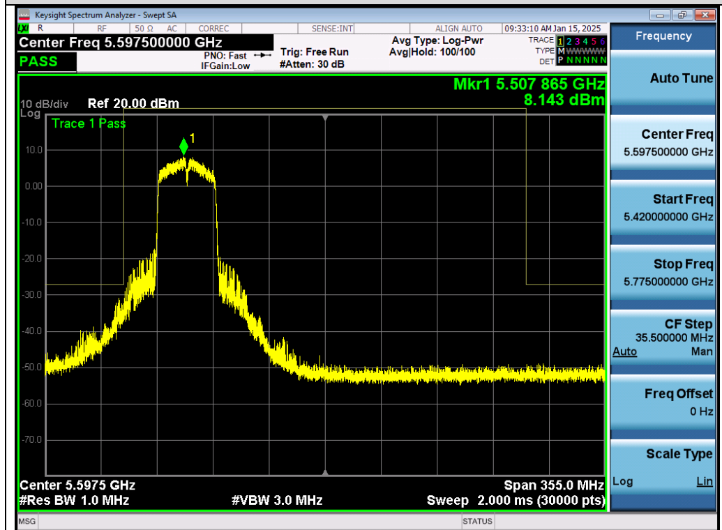
Test_Graph_802.11n40_Chain B_5510_MCS0_Frequency Band 3
