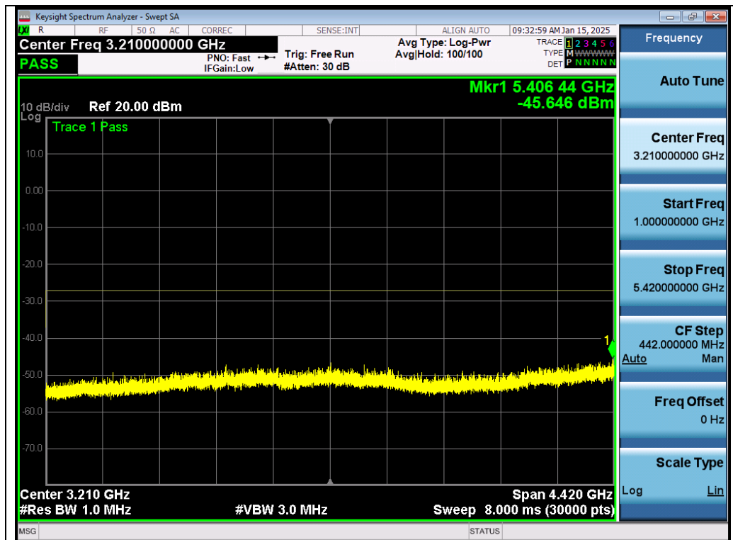
Test_Graph_802.11n40_Chain B_5510_MCS0_Frequency Band 2
