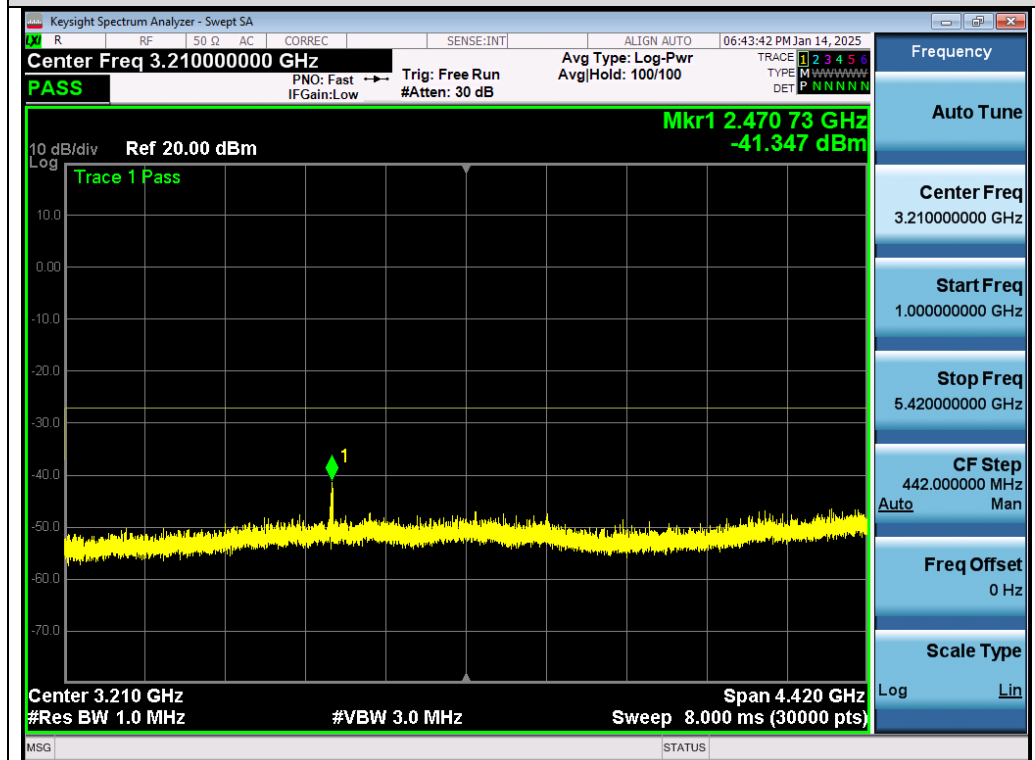
Test_Graph_802.11ax80_Chain A_5610_MCS0_Frequency Band 2
