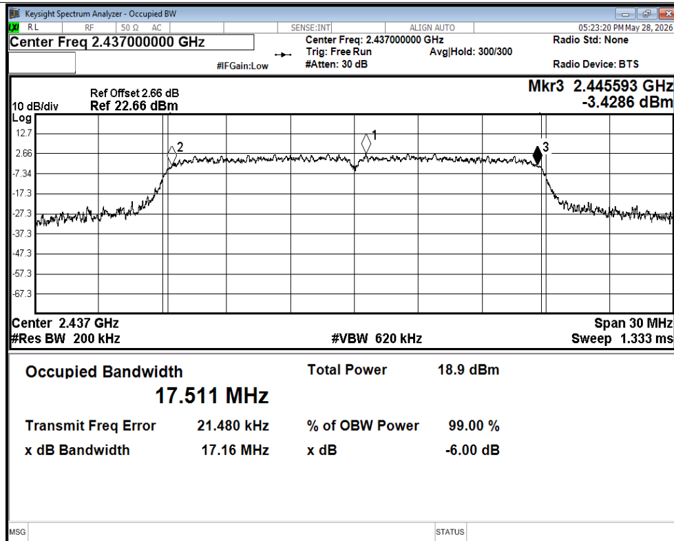
-6dB Bandwidth NVNT ax20 2437MHz Ant2
