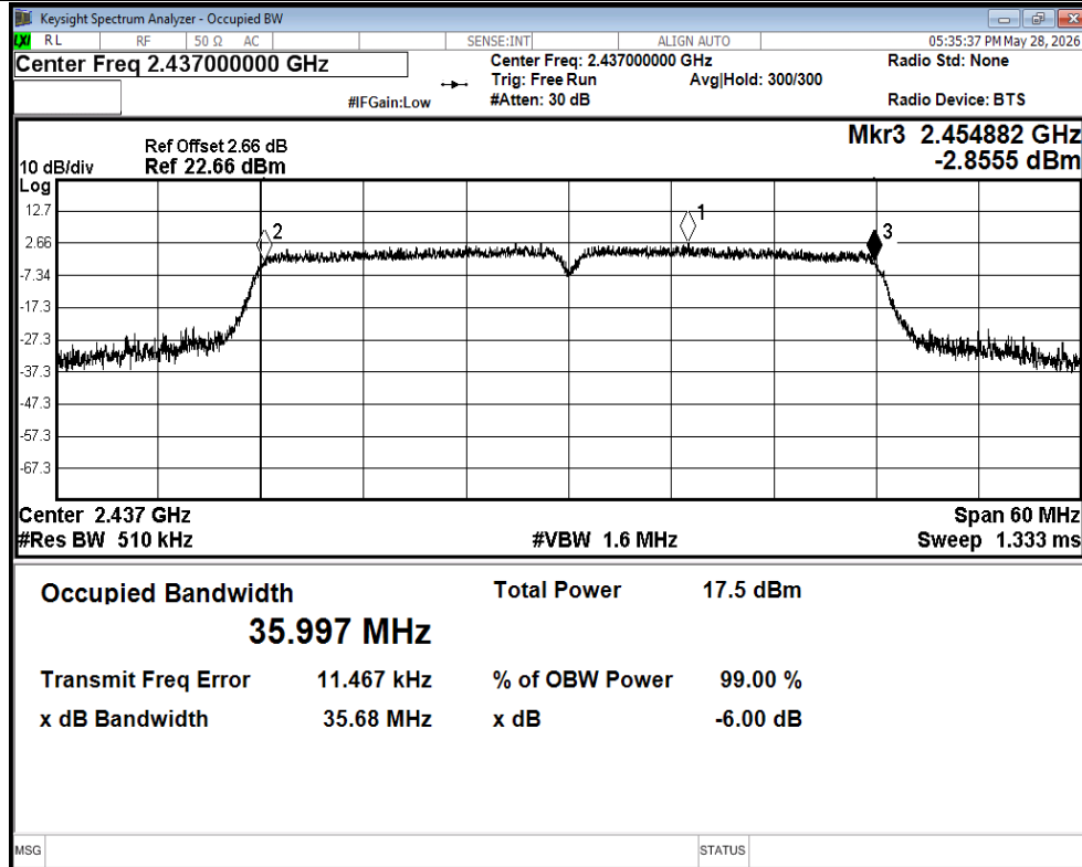
-6dB Bandwidth NVNT n40 2437MHz Ant2
