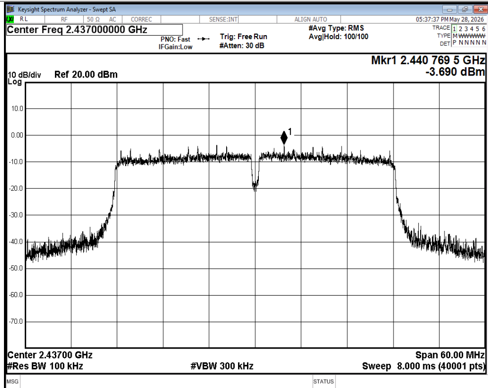
Tx. Spurious NVNT ax40 2437MHz Ant2 Ref
