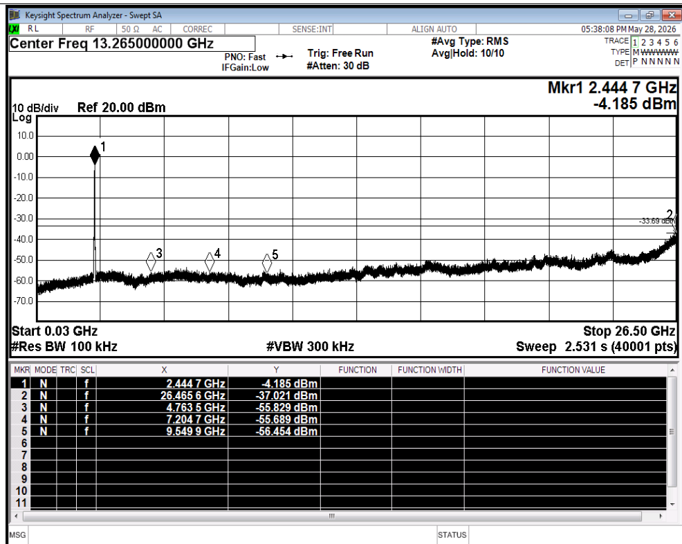
Tx. Spurious NVNT ax40 2437MHz Ant2 Emission
