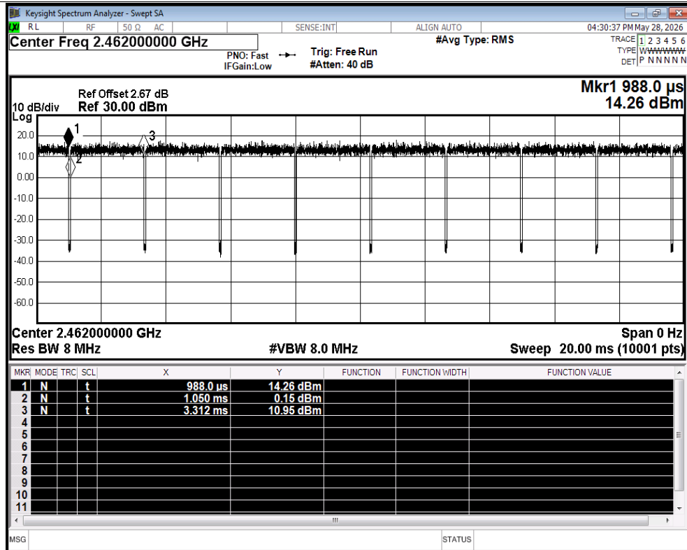
Duty Cycle NVNT ax20 2462MHz Ant1
