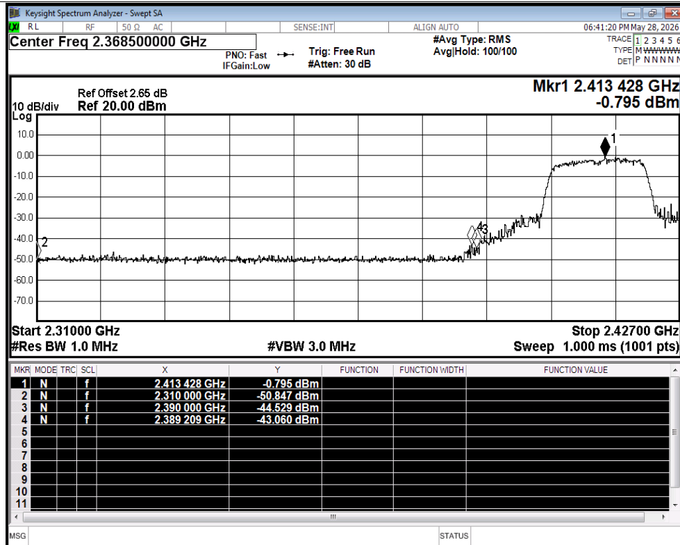
Restrict Band NVNT ax20 2412MHz Ant1 Peak
