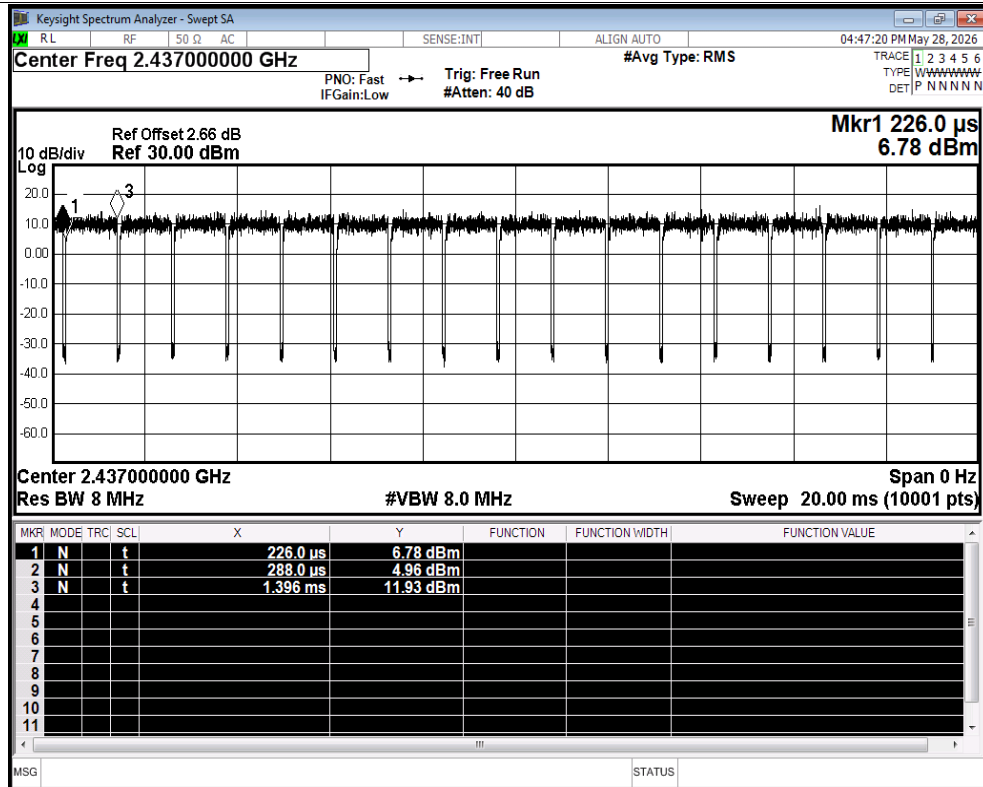
Duty Cycle NVNT ax40 2437MHz Ant1
