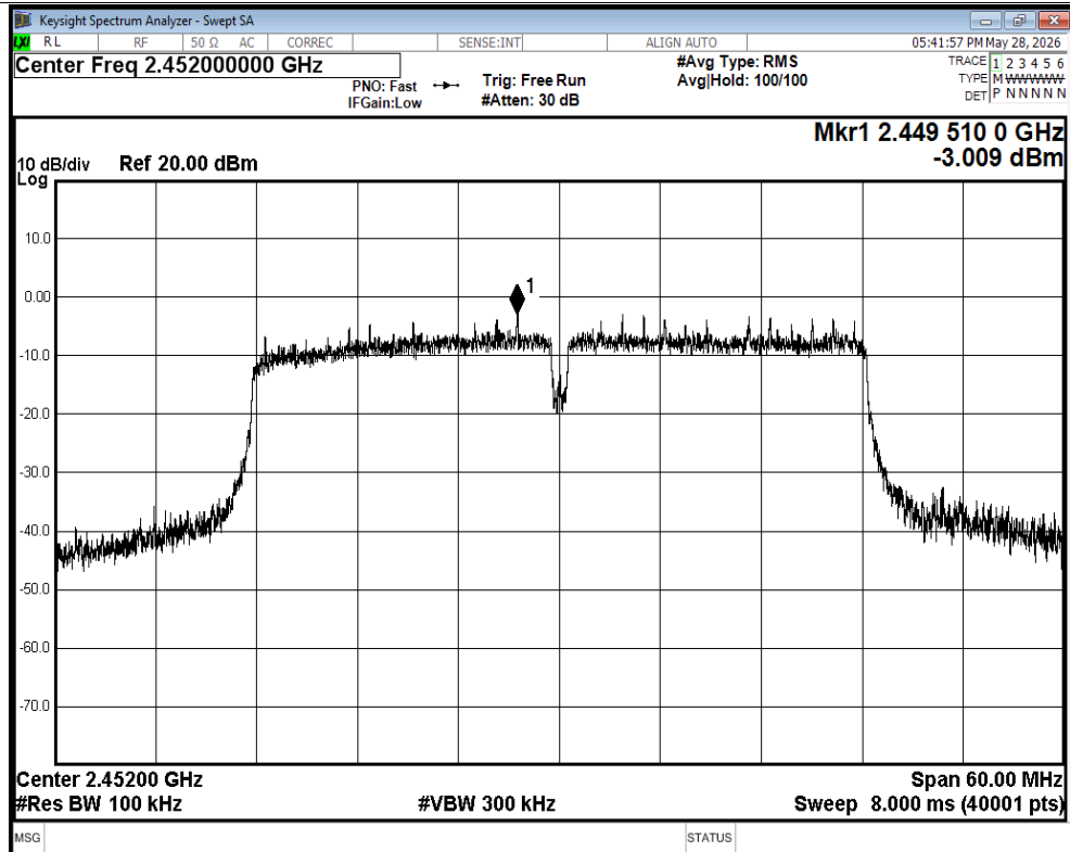
Tx. Spurious NVNT ax40 2452MHz Ant2 Ref
