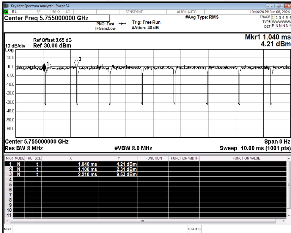
Duty Cycle NVNT ax40 5755MHz Ant2
