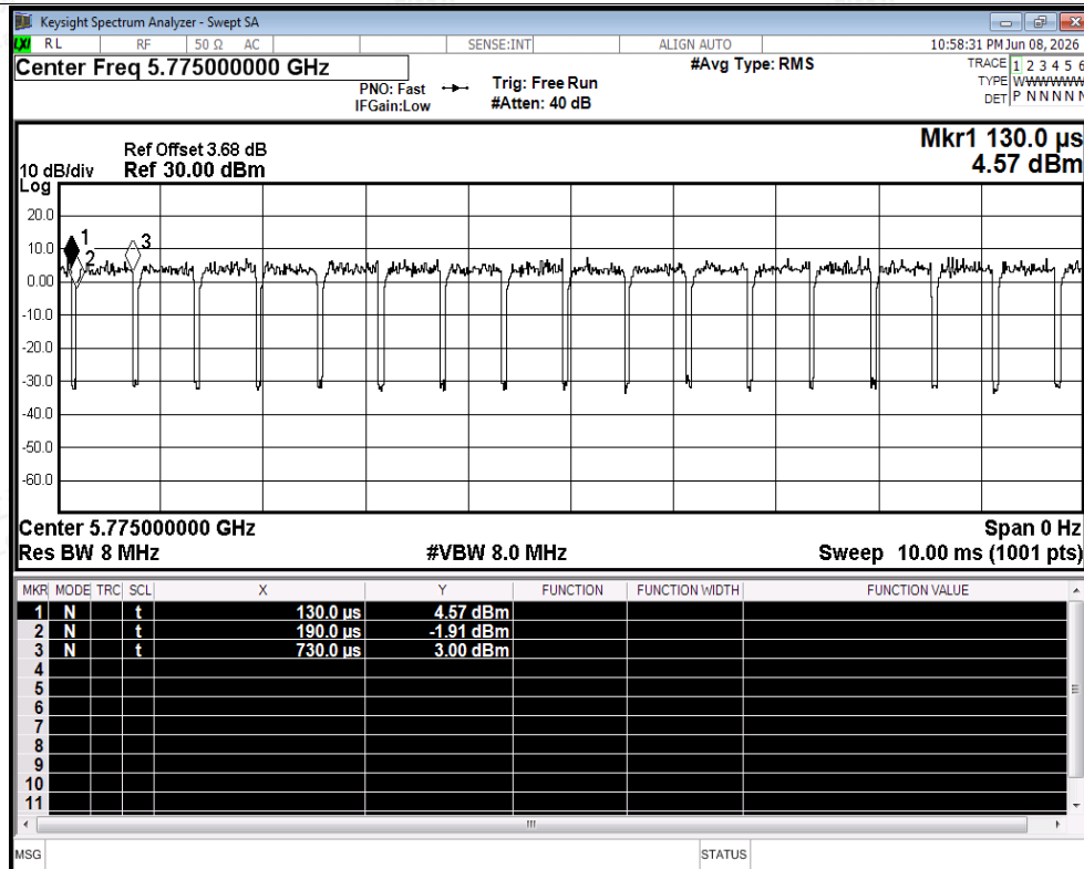
Duty Cycle NVNT ax80 5775MHz Ant2
