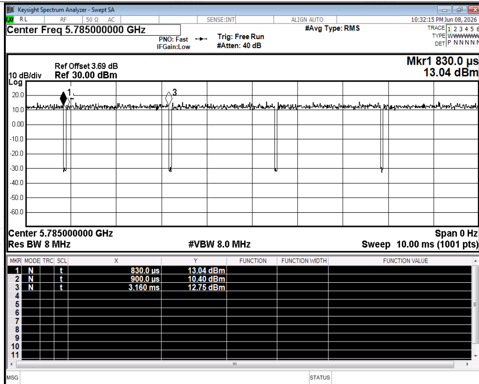
Duty Cycle NVNT ax20 5785MHz Ant2
