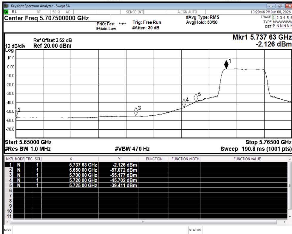
Restrict Band NVNT ax20 5745MHz Ant2 Average
