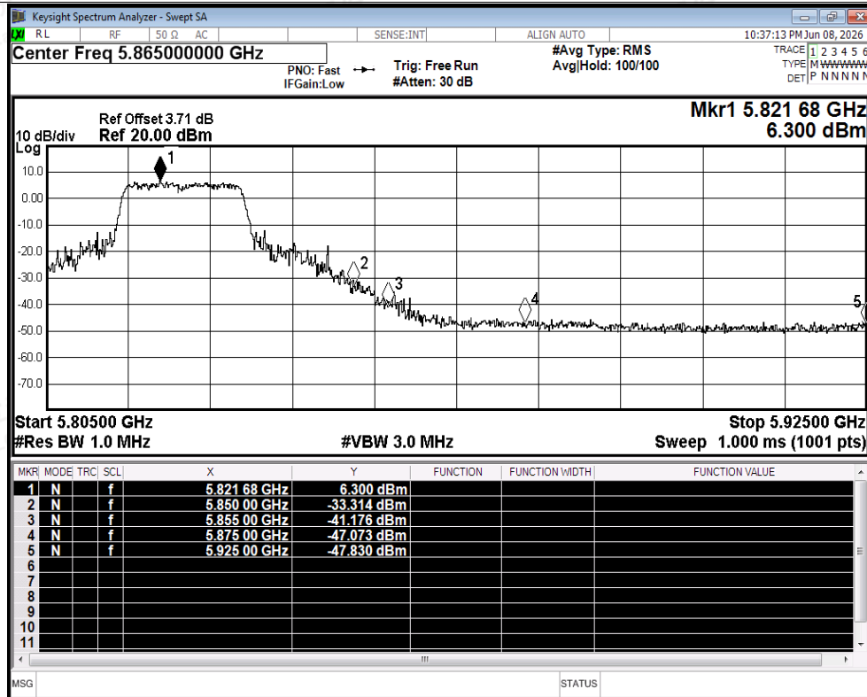
Restrict Band NVNT ax20 5825MHz Ant2 Peak
