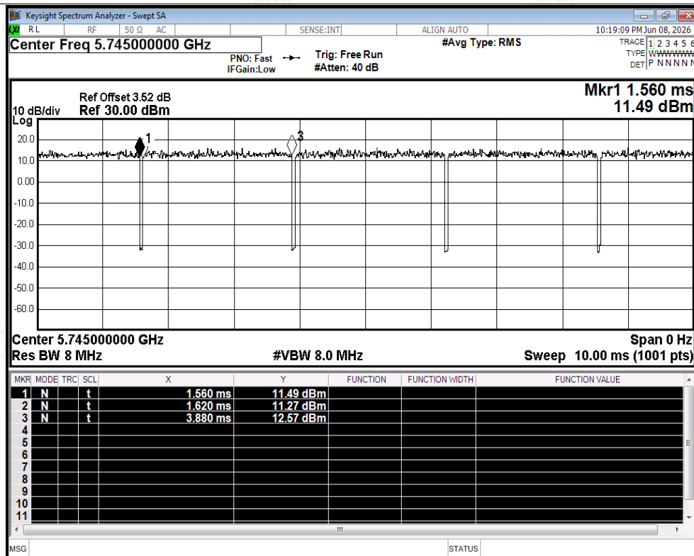
Duty Cycle NVNT n20 5745MHz Ant2
