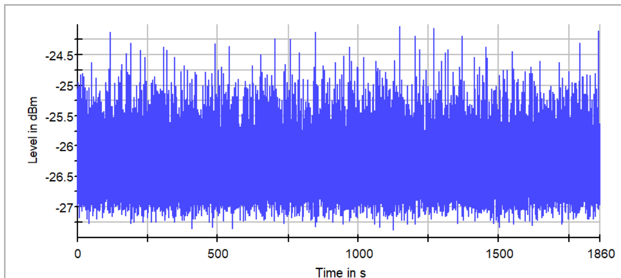
802.11a Channel 52
