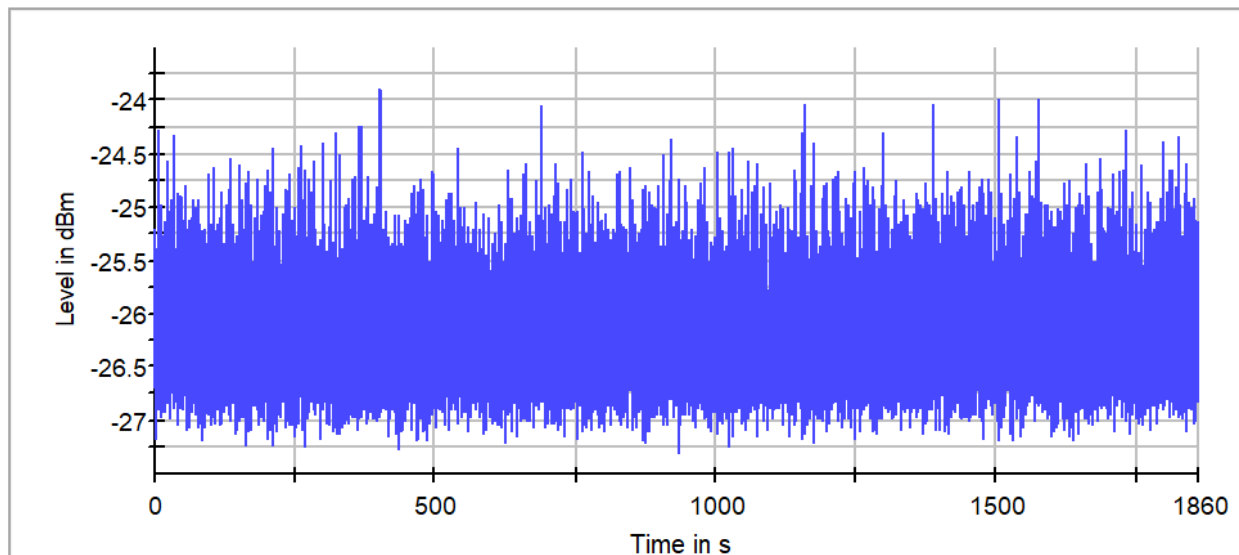
802.11a Channel 100
