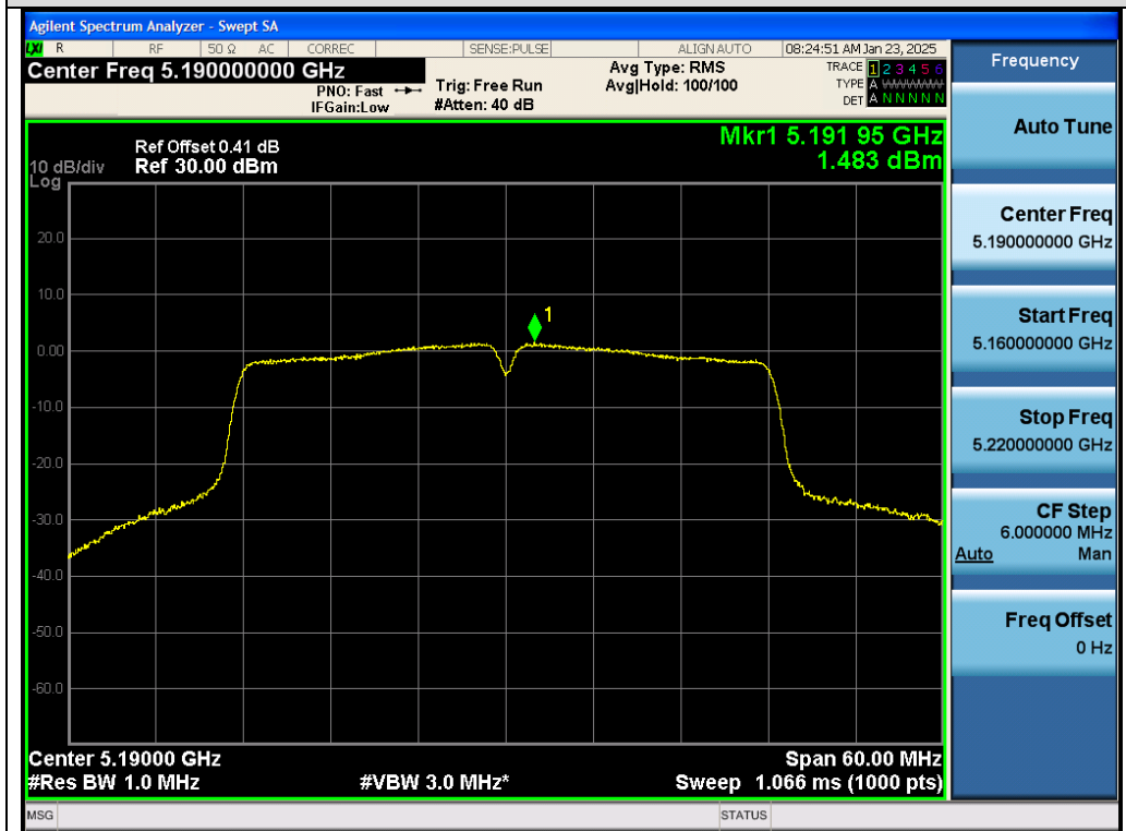
Test_Graph_802.11ac40_Chain B_5190_MCS0_PSD
