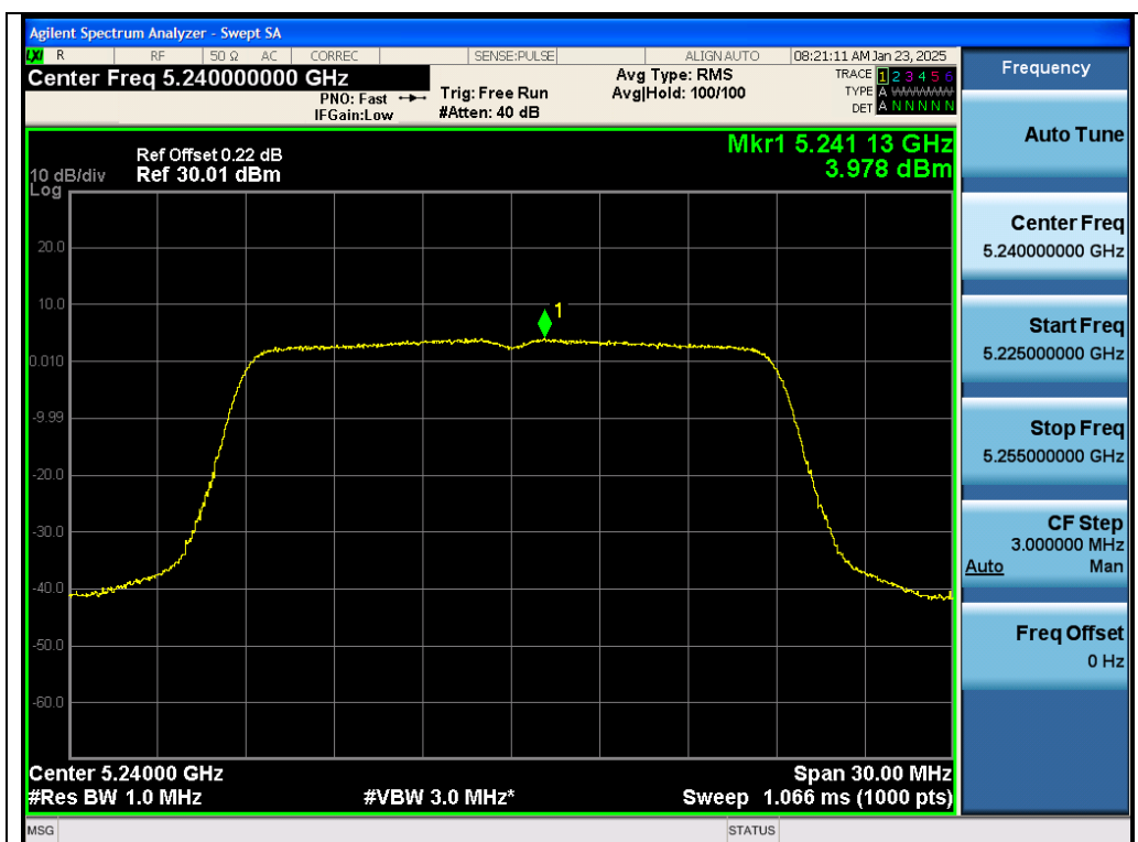
Test_Graph_802.11ac20_Chain B_5240_MCS0_PSD
