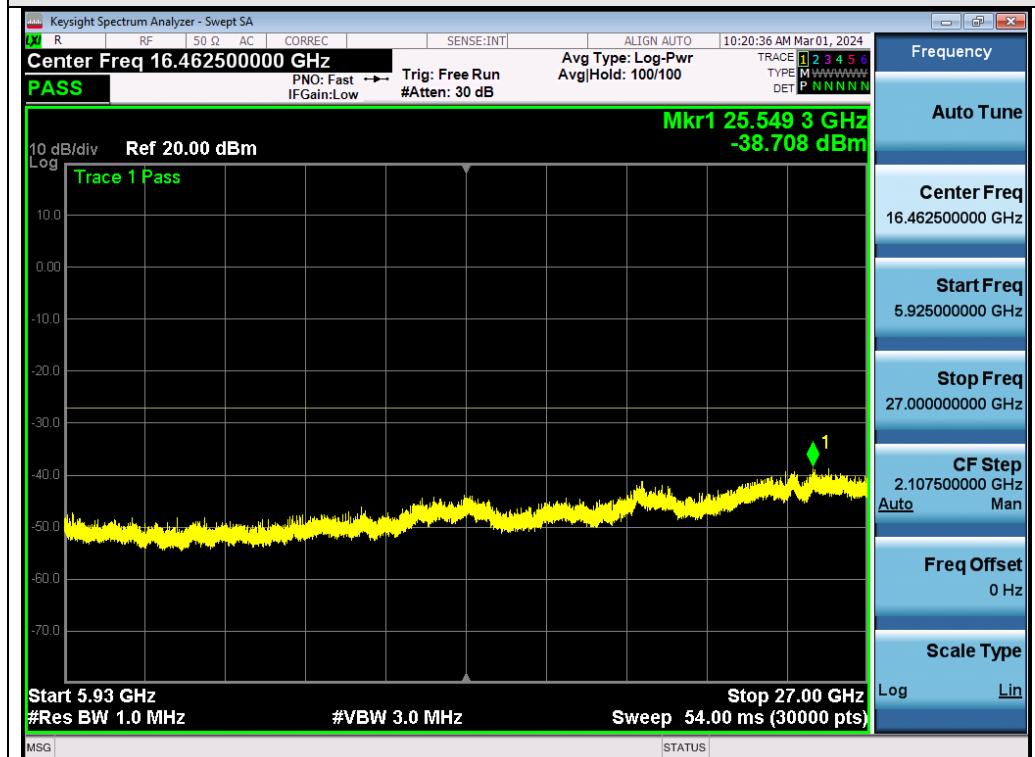
Test_Graph_802.11ac80_ANT2_5775_MCS9_Frequency Band4
