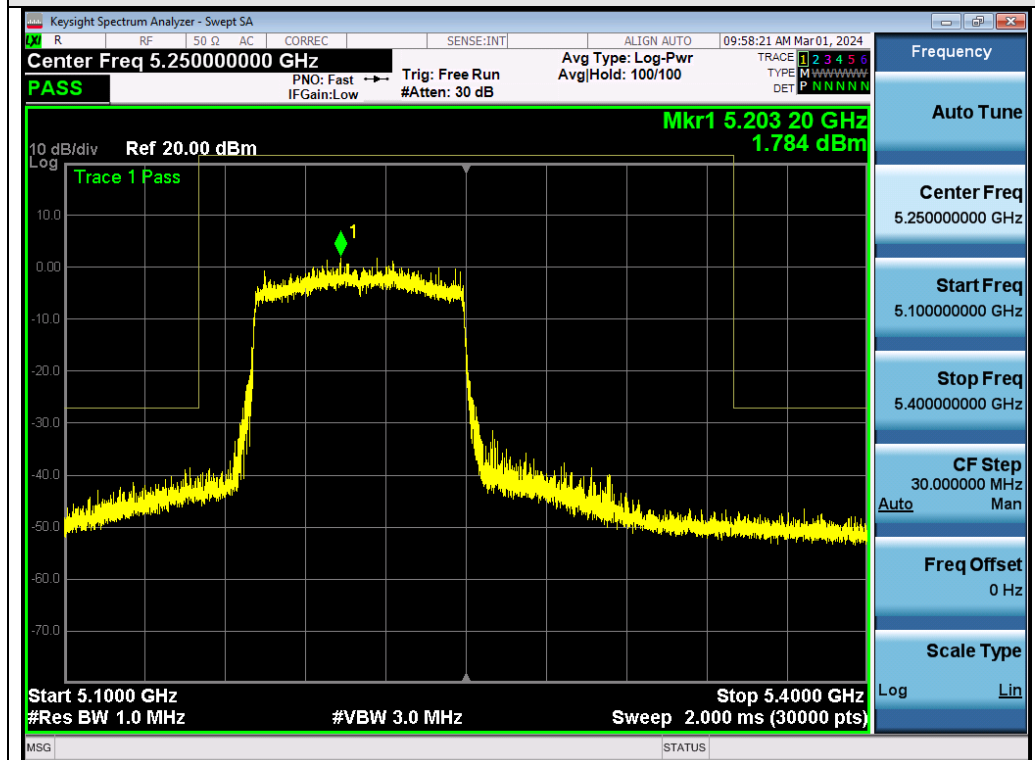
Test_Graph_802.11ax80_ANT2_5210_MCS0_Frequency Band 3
