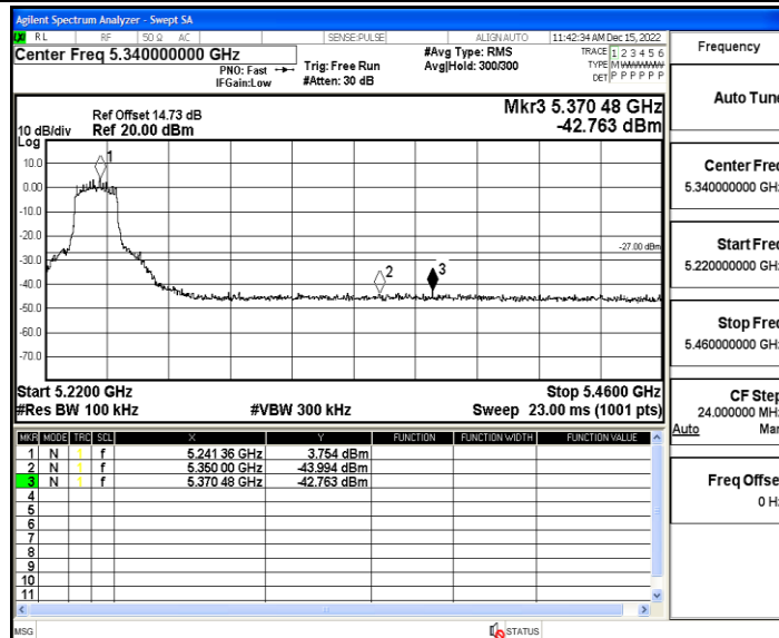
11A_Ant2_High_5240
