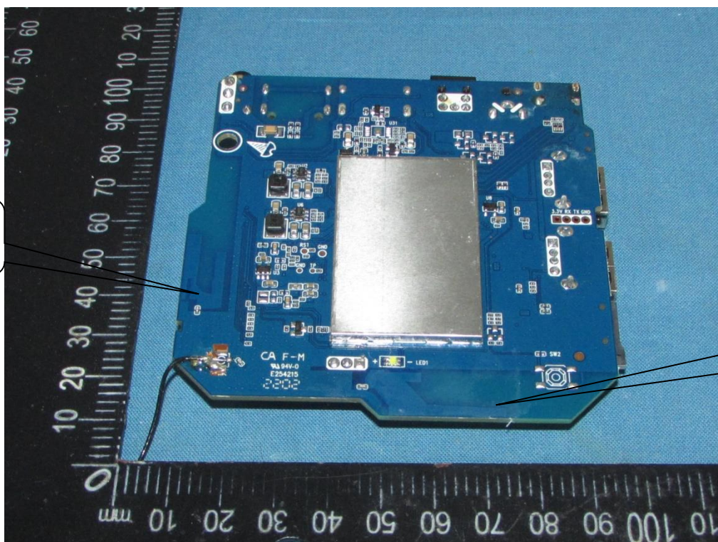
WiFi Antenna 2
