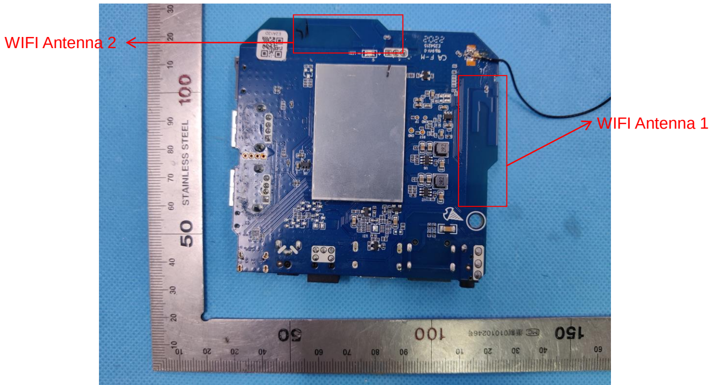
INTERNAL VIEW OF EUT (FIGURE 2)
