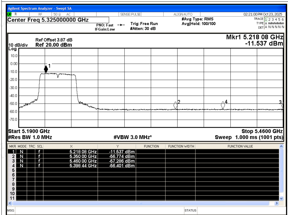
Restrict Band NVNT n40 5230MHz Ant1 Average
