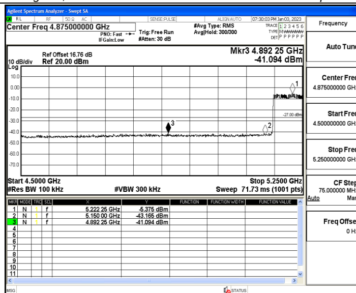
11AX80MIMO_Ant1_High_5210
