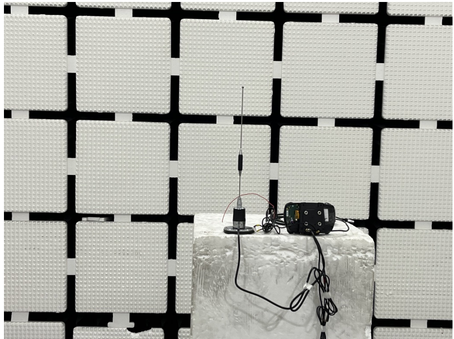
Radiation Emission Test Setup
