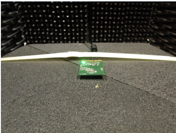
Module on Dev Board Flat EUT Orientation for Radiated Tests
