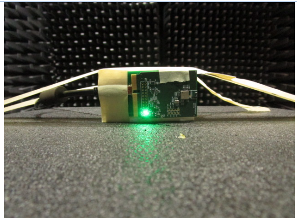
Module on Dev Board Horizontal EUT Orientation for Radiated Tests
