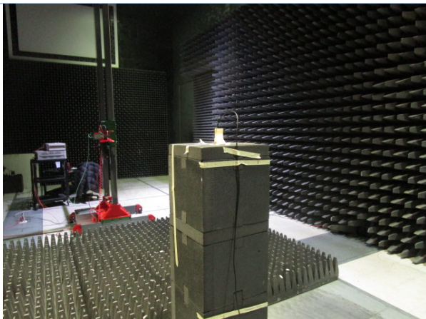
Radiated Emissions 4-25 GHz, Rear View
