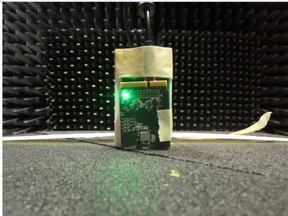
Module on Dev Board Vertical EUT Orientation for Radiated Tests
