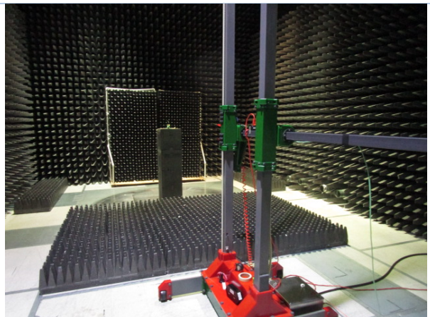
Radiated Emissions 4-25 GHz, Front View
