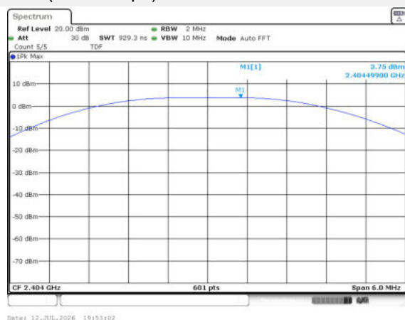
GFSK (BLE 2Mbps) LOW CHANNEL
