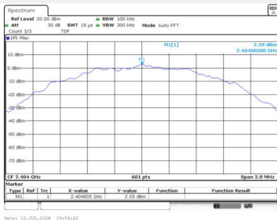
GFSK (BLE 2Mbps) LOW CHANNEL, CARRIER LEVEL
