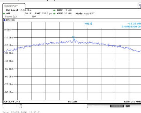
GFSK (BLE 2Mbps) MIDDLE CHANNEL
