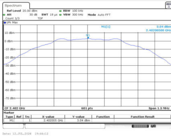
GFSK (BLE 1Mbps) LOW CHANNEL, CARRIER LEVEL
