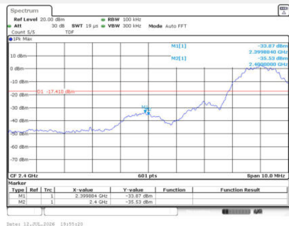
GFSK (BLE 2Mbps) LOW CHANNEL, BAND EDGE
