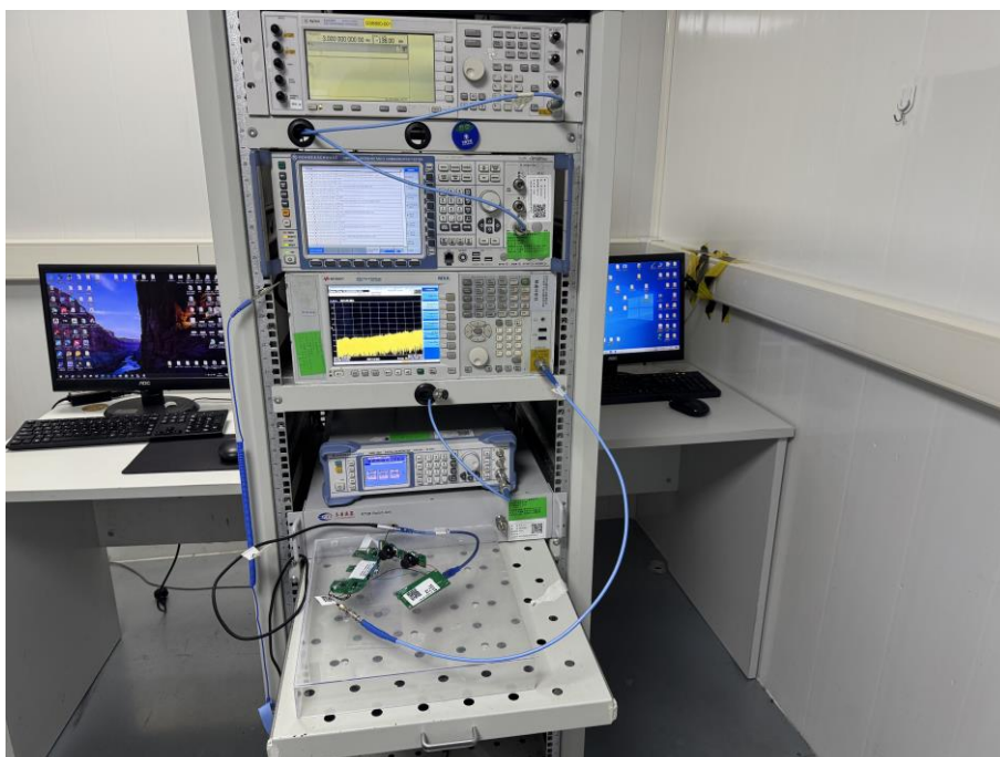
Conducted Test-BT/2.4G ISM Band
