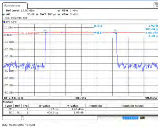
GFSK DH1
