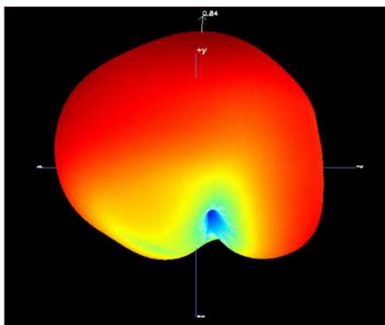
B1.2 3D Pattern for 2440MHz
