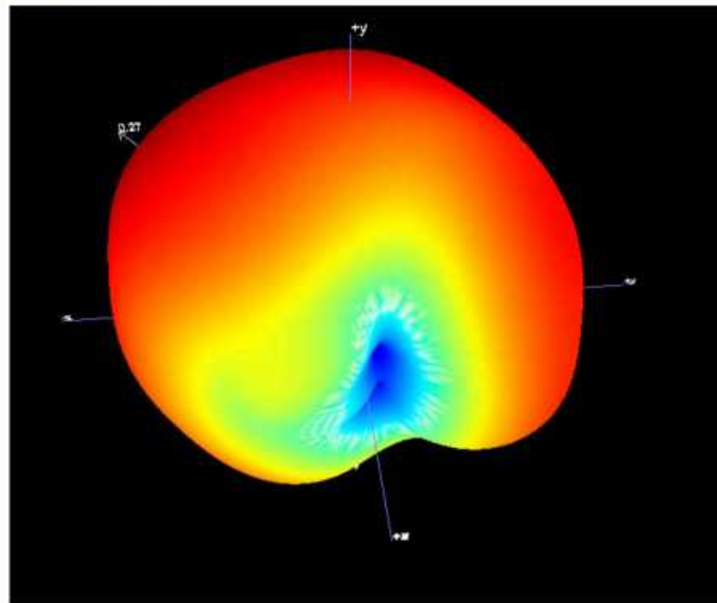
B1.3 3D Pattern for 2480MHz
