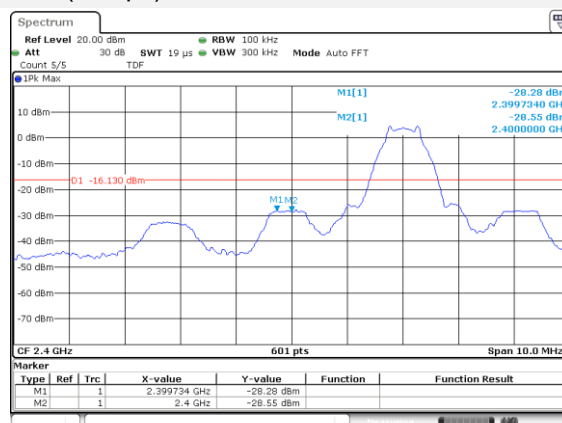
GFSK (1Mbps) LOW CHANNEL, BAND EDGE
