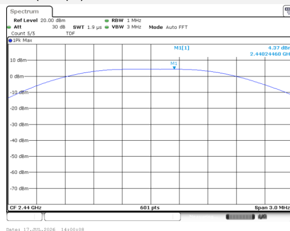
GFSK (1Mbps) MIDDLE CHANNEL
