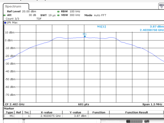
GFSK (1Mbps) LOW CHANNEL, CARRIER LEVEL
