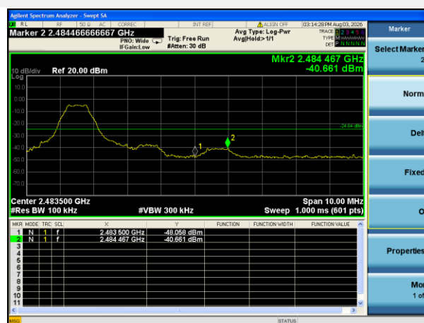
GFSK (1Mbps) HIGH CHANNEL, BAND EDGE
