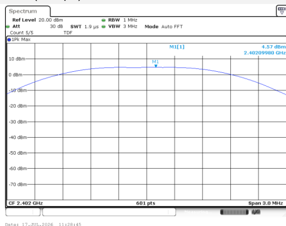
GFSK (1Mbps) LOW CHANNEL
