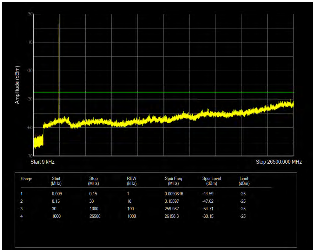
Band41 QPSK BW=5MHz Channel=40715 RB Size=25 Position=#0
