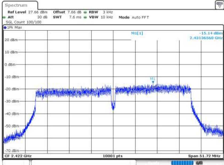
PSD NVNT 802.11n(HT40) 2422MHz Ant1
