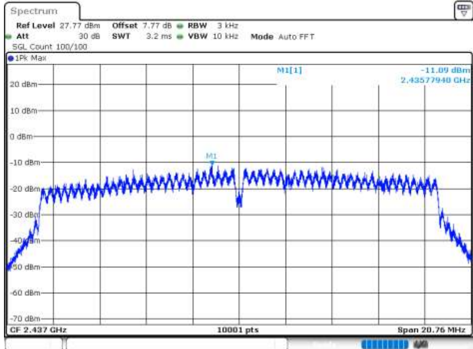
PSD NVNT 802.11n(HT20) 2437MHz Ant1
