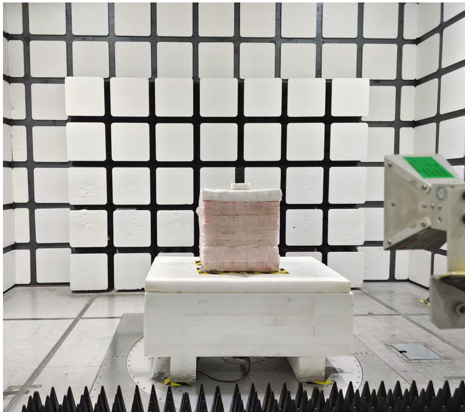
Radiated Emissions View (18-25 GHz)
