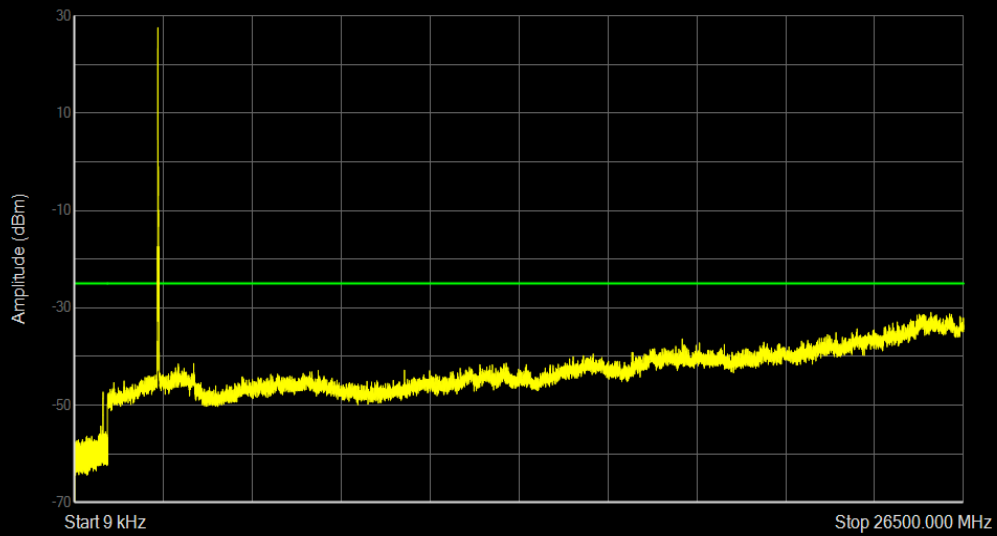
Band7 QAM16 BW=20MHz Channel=20850 RB Size=1 Position=#0
