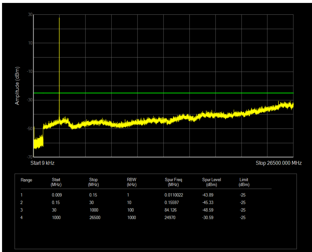
Band41(2540-2650) QPSK BW=5MHz Channel=41165 RB Size=25 Position=#0
