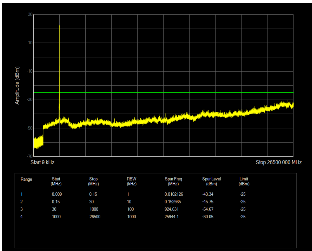
Band41(2540-2650) QAM16 BW=10MHz Channel=41140 RB Size=1 Position=#0
