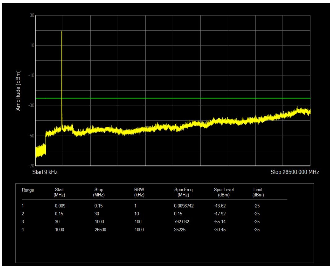
Band41(2540-2650) QPSK BW=15MHz Channel=40640 RB Size=1 Position=#0
