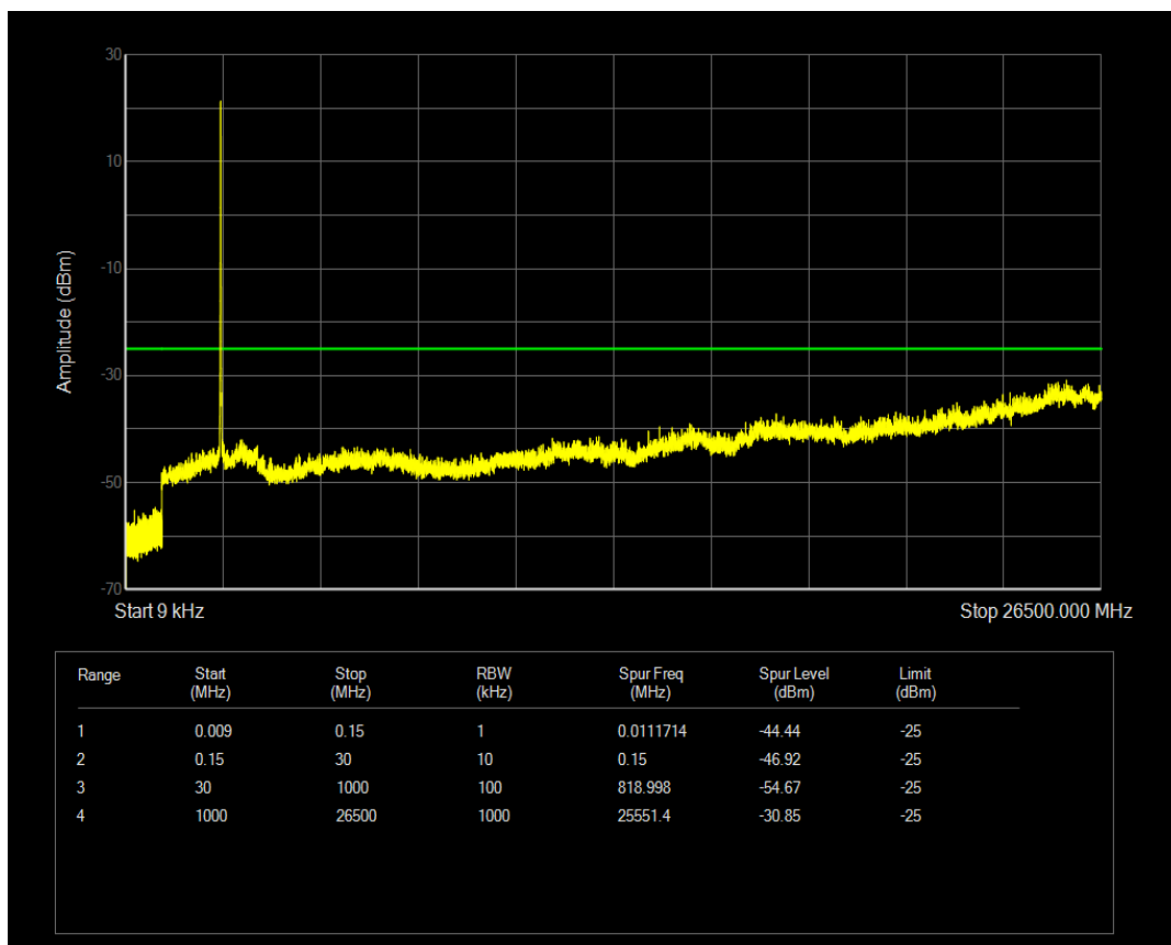
Band41(2540-2650) QAM16 BW=10MHz Channel=40640 RB Size=1 Position=#0
