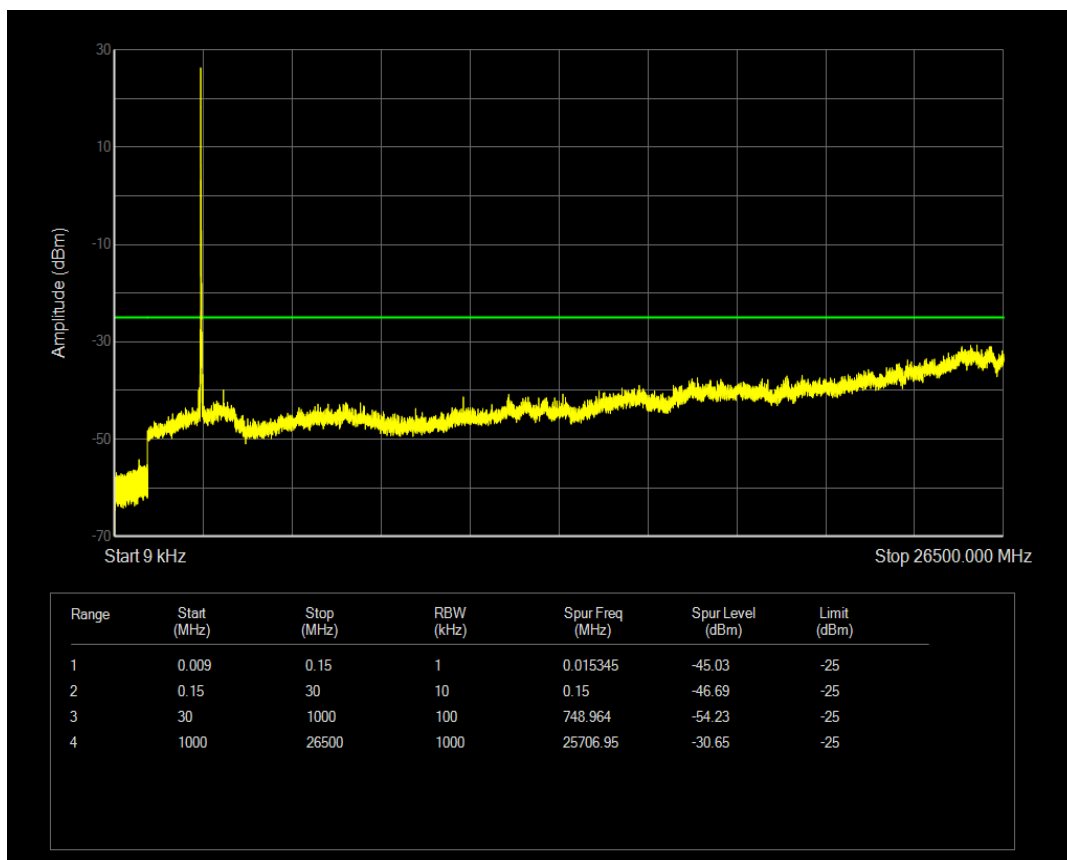
Band41(2540-2650) QPSK BW=20MHz Channel=40640 RB Size=100 Position=#0
