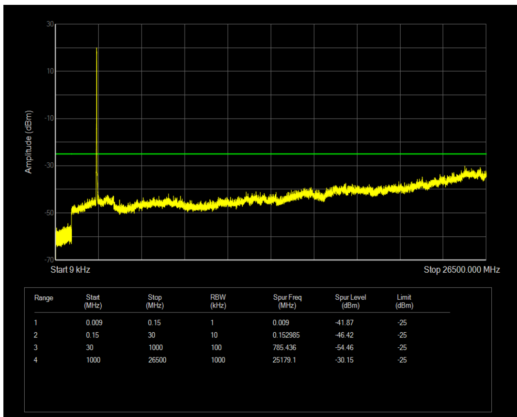
Band41(2540-2650) QPSK BW=20MHz Channel=40640 RB Size=1 Position=#0
