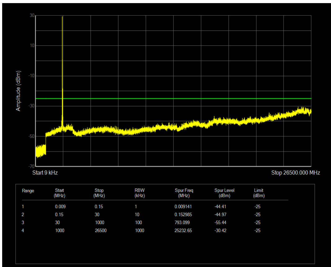
Band41(2540-2650) QAM16 BW=20MHz Channel=40640 RB Size=100 Position=#0
