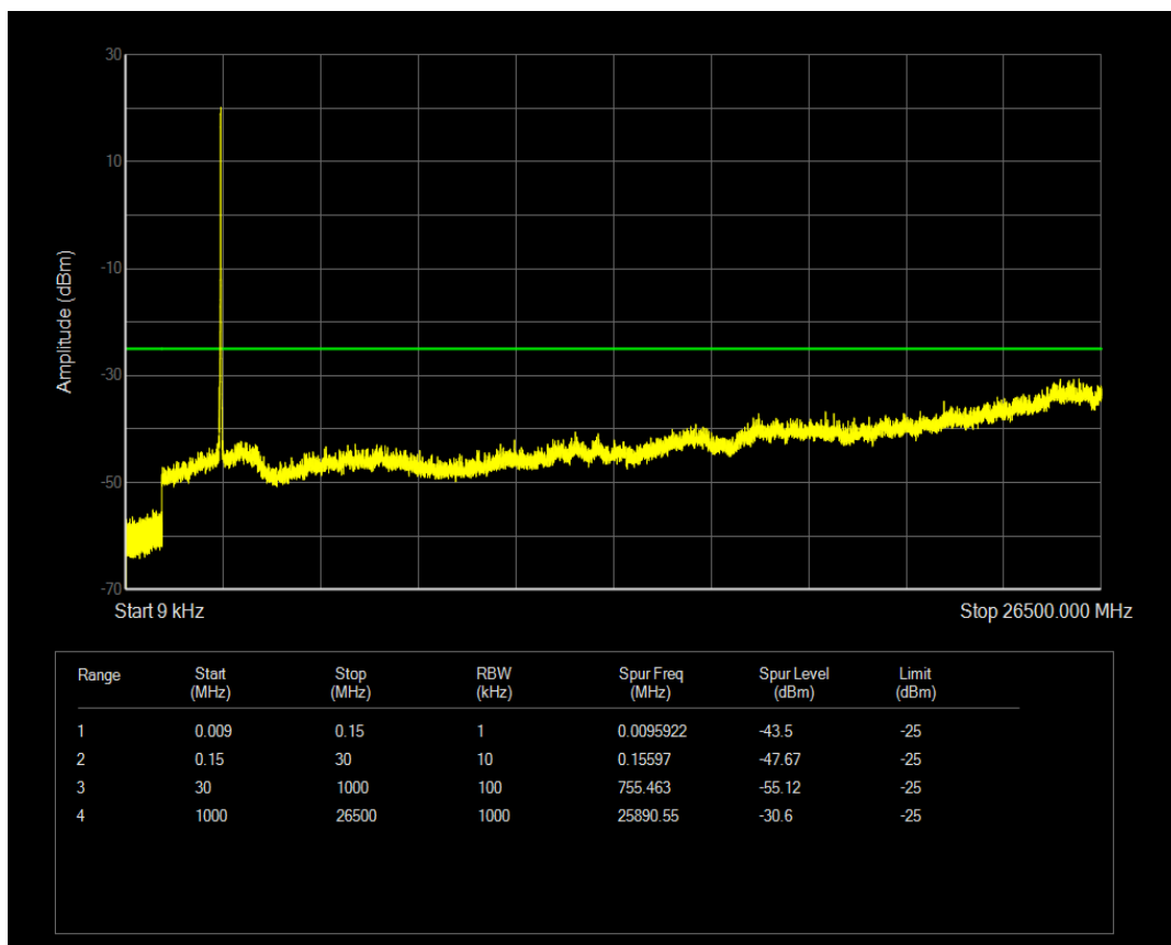
Band41(2540-2650) QPSK BW=15MHz Channel=41115 RB Size=1 Position=#0
