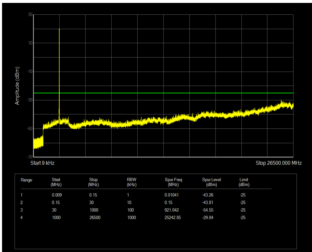
Band41(2540-2650) QPSK BW=15MHz Channel=40165 RB Size=1 Position=#0
