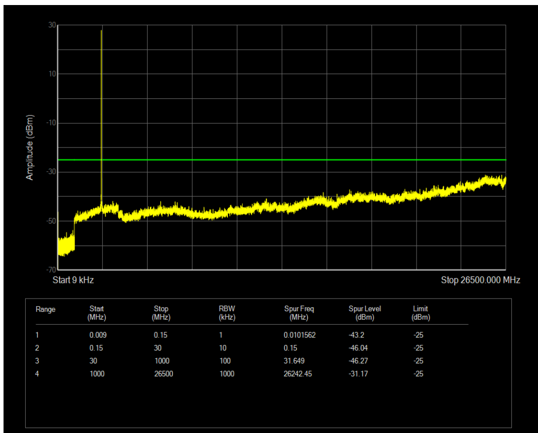
Band41(2540-2650) QPSK BW=5MHz Channel=40640 RB Size=25 Position=#0
