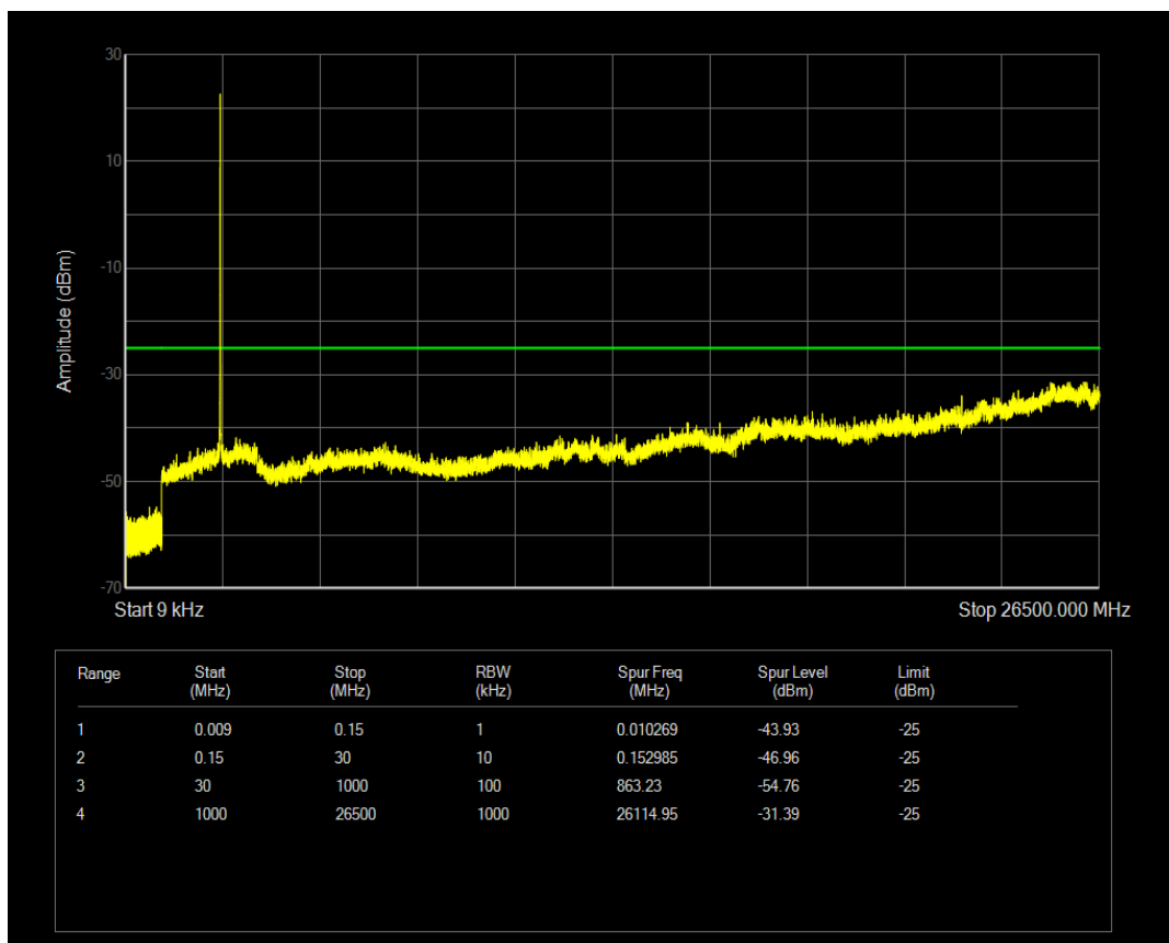
Band41(2540-2650) QPSK BW=5MHz Channel=41165 RB Size=1 Position=#0
