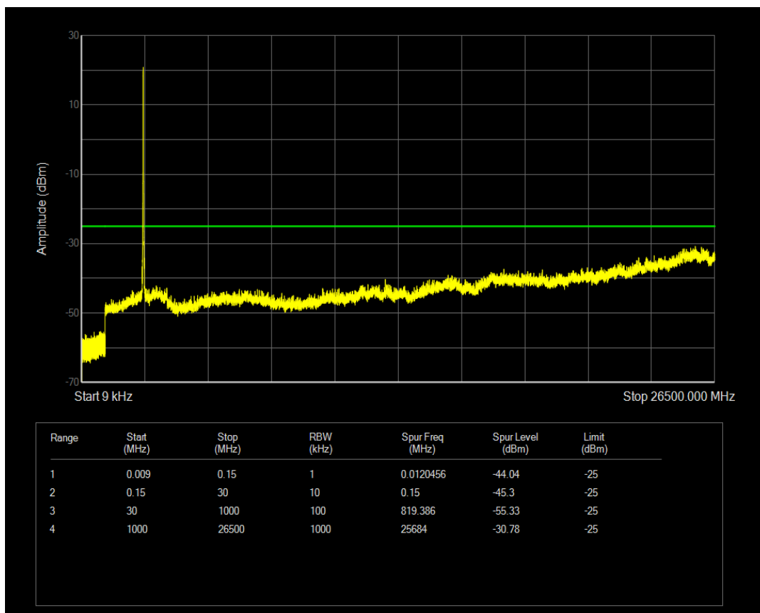
Band41(2540-2650) QAM16 BW=15MHz Channel=40640 RB Size=1 Position=#0
