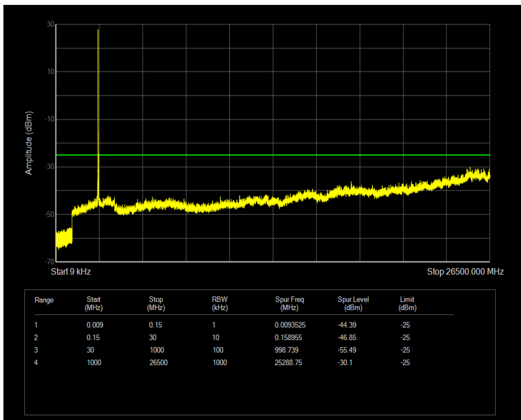
Band41(2540-2650) QAM16 BW=15MHz Channel=40640 RB Size=75 Position=#0
