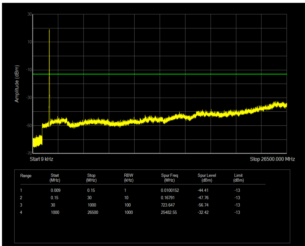
Band41(2540-2650) QPSK BW=5MHz Channel=40115 RB Size=1 Position=#0
