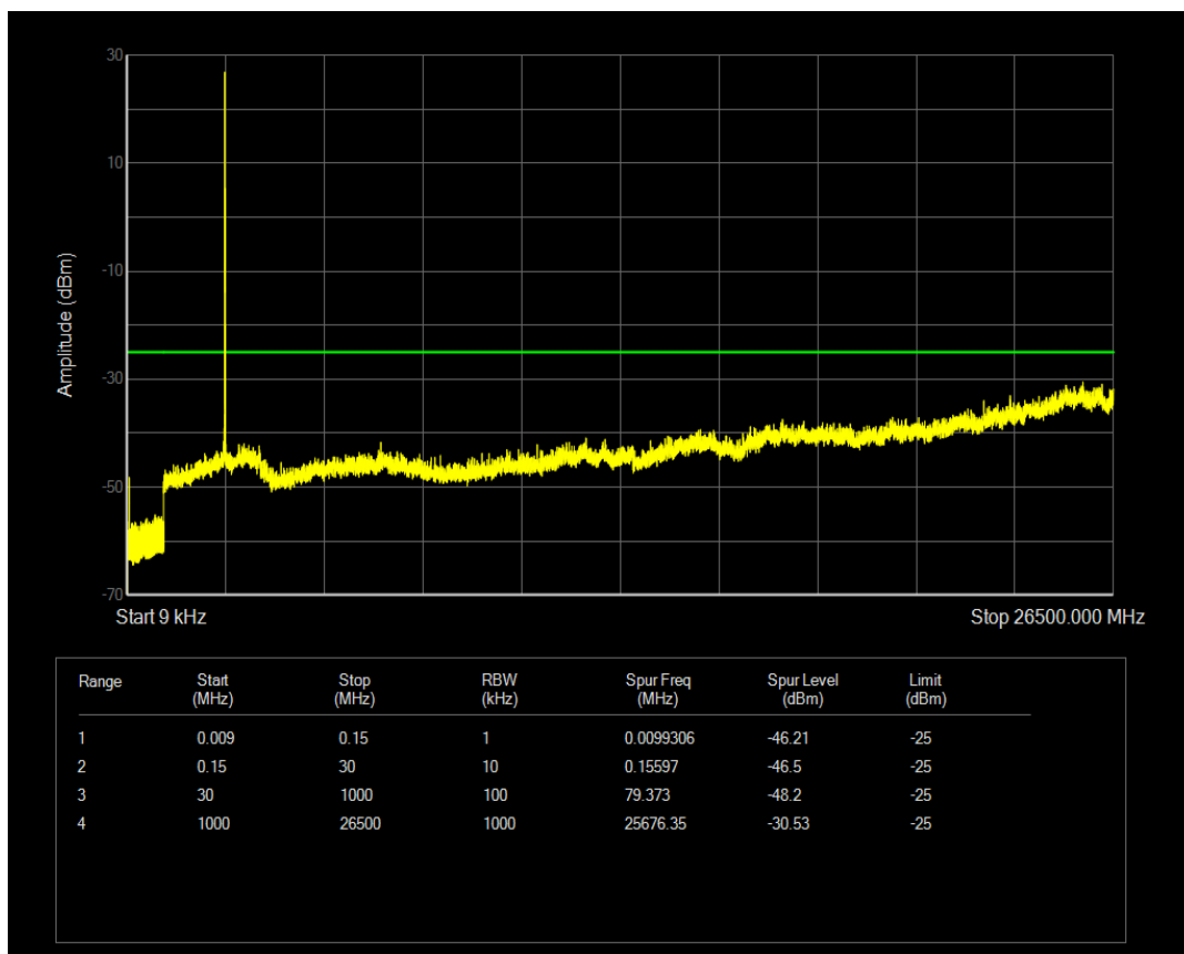
Band41(2540-2650) QPSK BW=10MHz Channel=41140 RB Size=50 Position=#0
