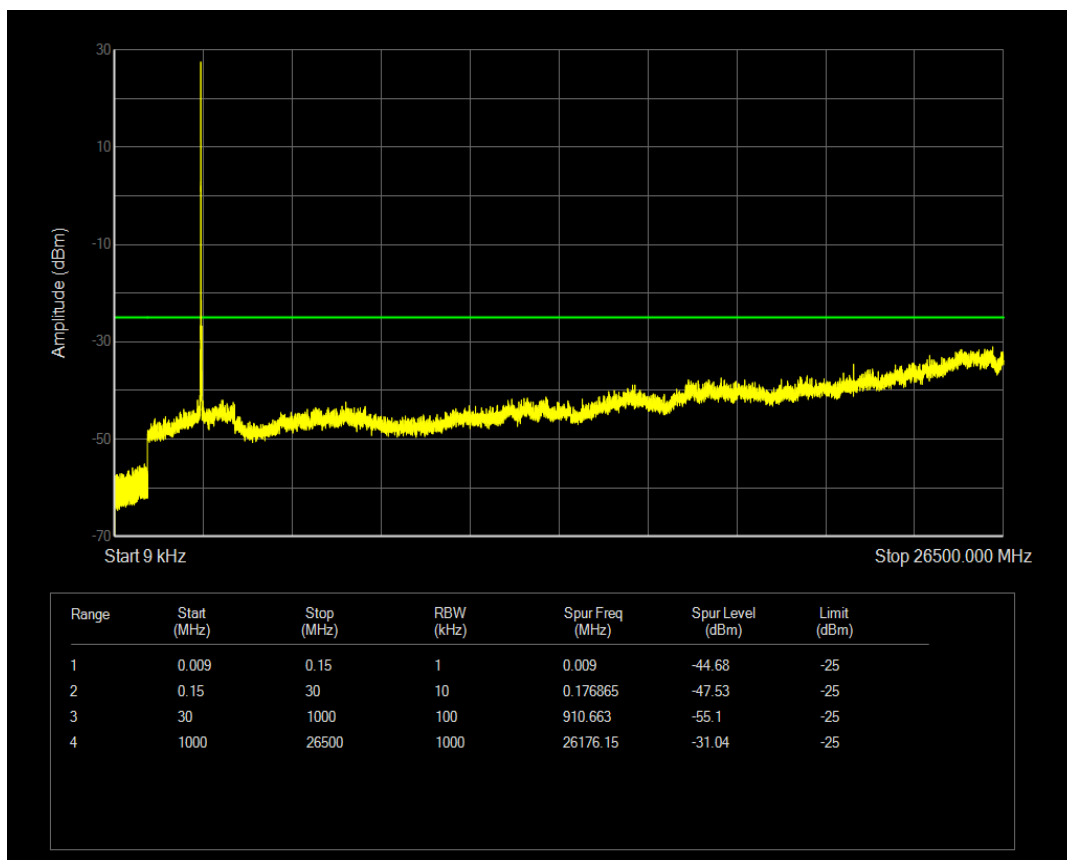
Band41(2540-2650) QPSK BW=15MHz Channel=40640 RB Size=75 Position=#0
