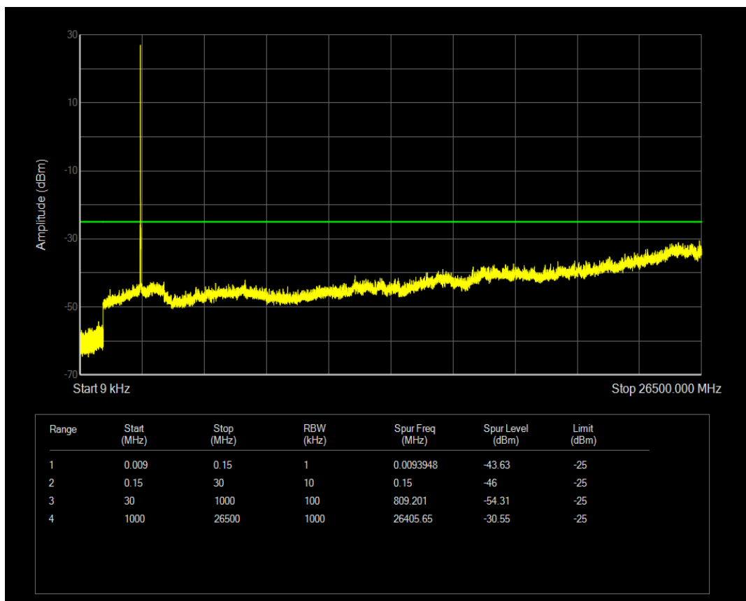
Band41(2540-2650) QAM16 BW=10MHz Channel=40640 RB Size=50 Position=#0
