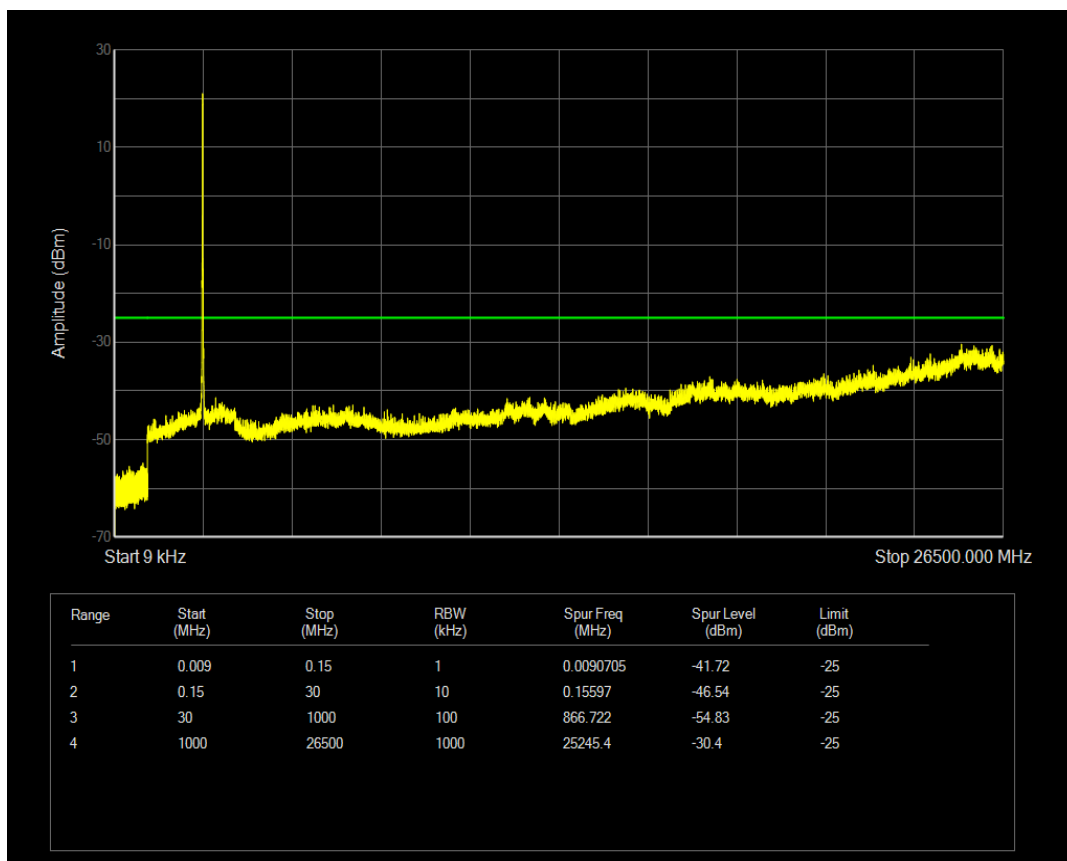
Band41(2540-2650) QPSK BW=20MHz Channel=40190 RB Size=1 Position=#0
