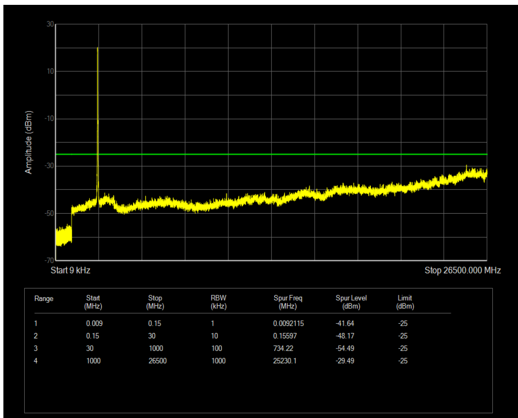
Band41(2540-2650) QAM16 BW=20MHz Channel=40640 RB Size=1 Position=#0
