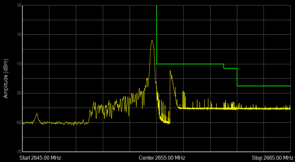
Band41(2535-2655) 16QAM BW=5MHz Channel=41215 RB Size=1 Position=#Max
