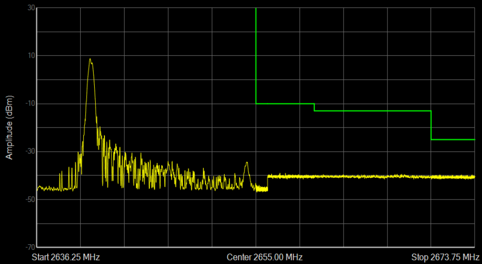
Band41(2535-2655) 16QAM BW=15MHz Channel=41165 RB Size=1 Position=#0
