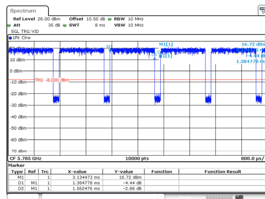
802.11a_5785MHz
