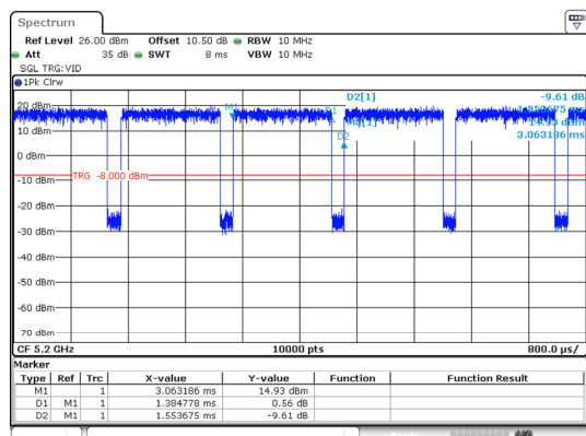
802.11a_5200MHz
