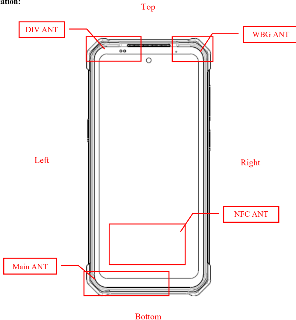
EUT Front View
