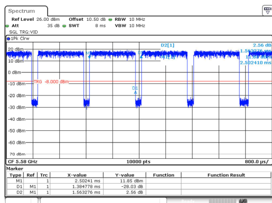
802.11a_5580MHz
