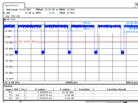
802.11a_5280MHz
