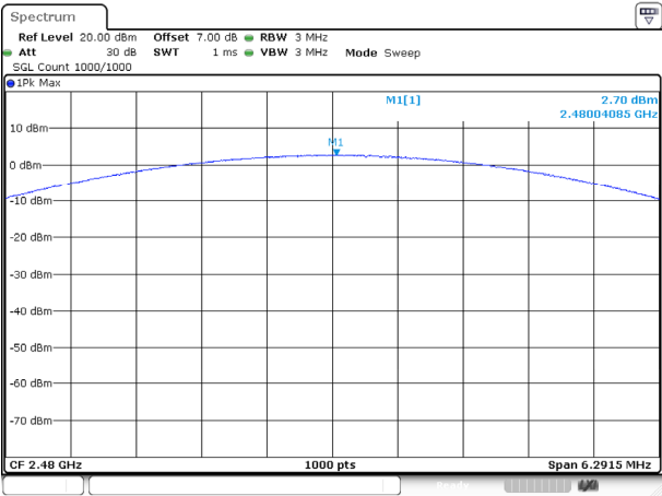
3DH1_High
