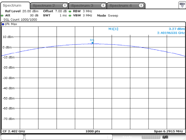
3DH1_Low
