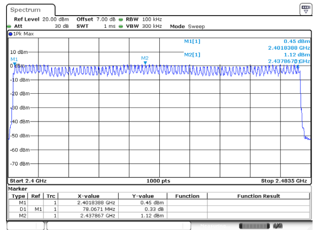
3DH1_Hopping
