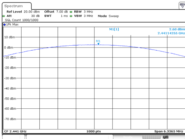
2DH1_Middle
