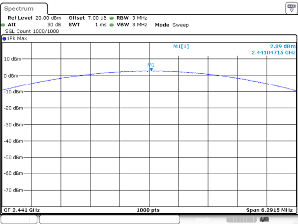
3DH1_Middle
