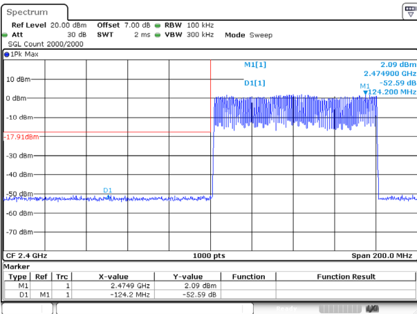
DH1_Hopping_Lower
