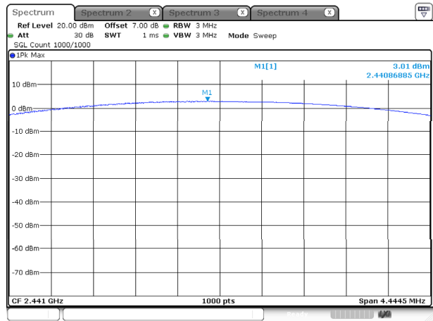
DH1_Middle
