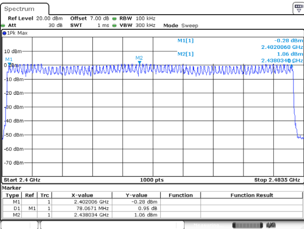
2DH1_Hopping
