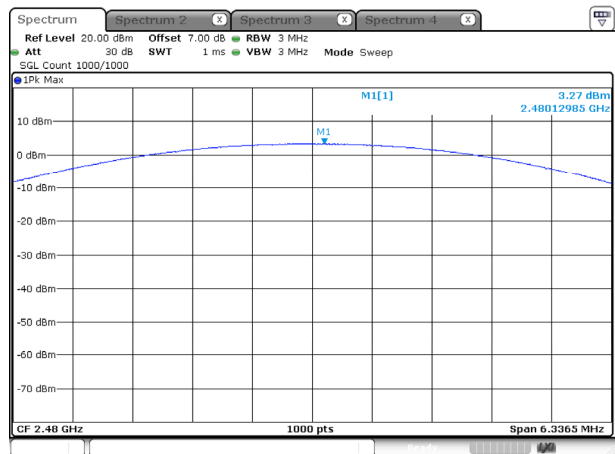
2DH1_High
