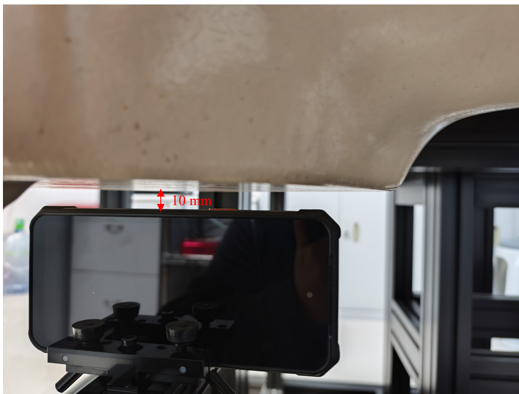
Main Ant Body Bottom Setup Photo (10 mm)
