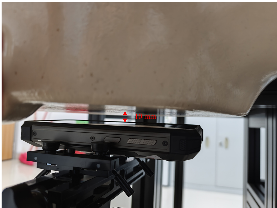
Main Ant Body Back Setup Photo (10 mm)
